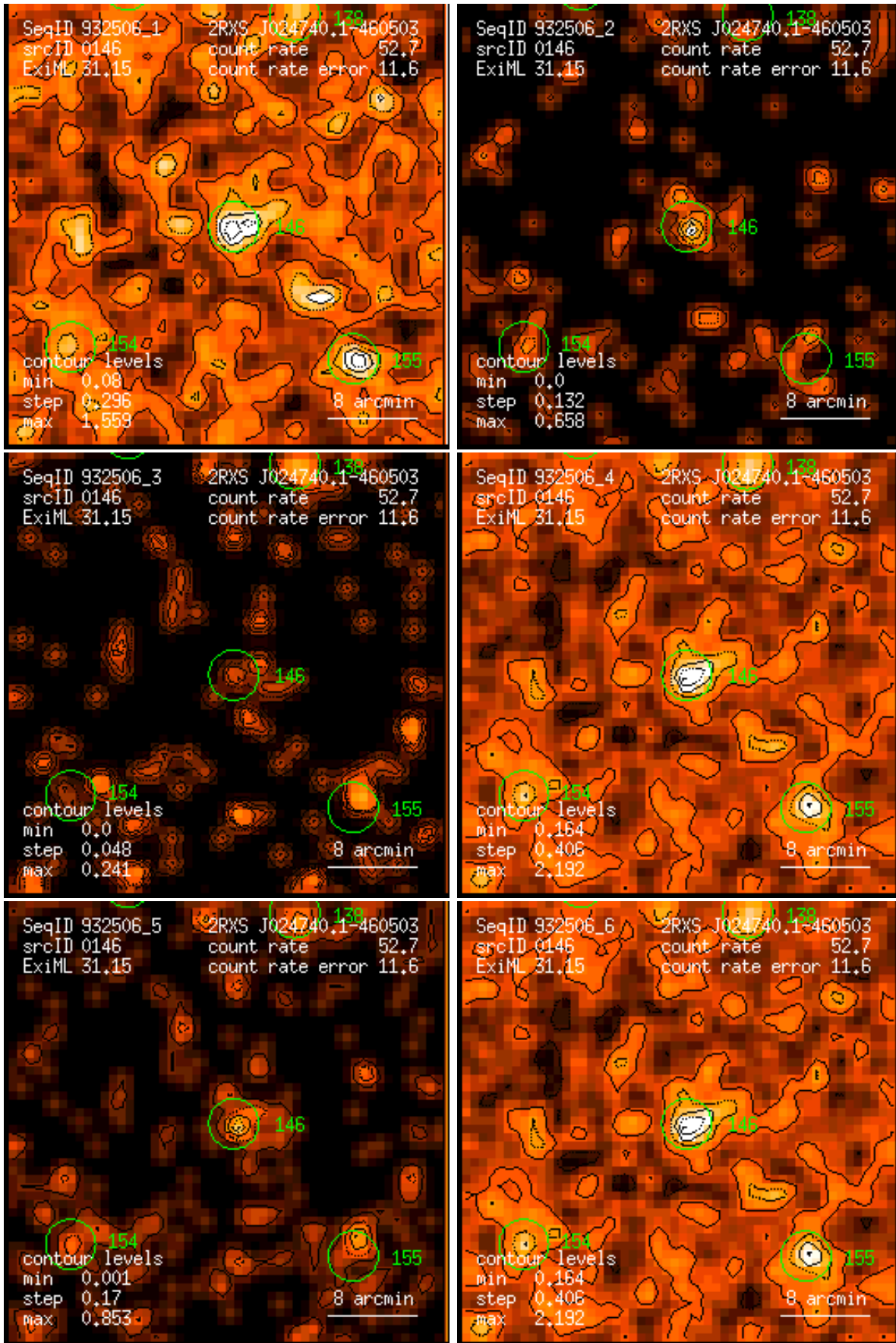
Figure 146: RASS 932506: detection 0146: band rate images, Gaussian filter: (1) PSPC channels 11 – 41, (2) 52 – 90, (3) 91 – 201, (4) 11 – 235, (5) 52 – 201, (6) 11 – 201. Broad band rates in counts/ks. Band rate contour levels in counts/ks/arcmin 2 .
