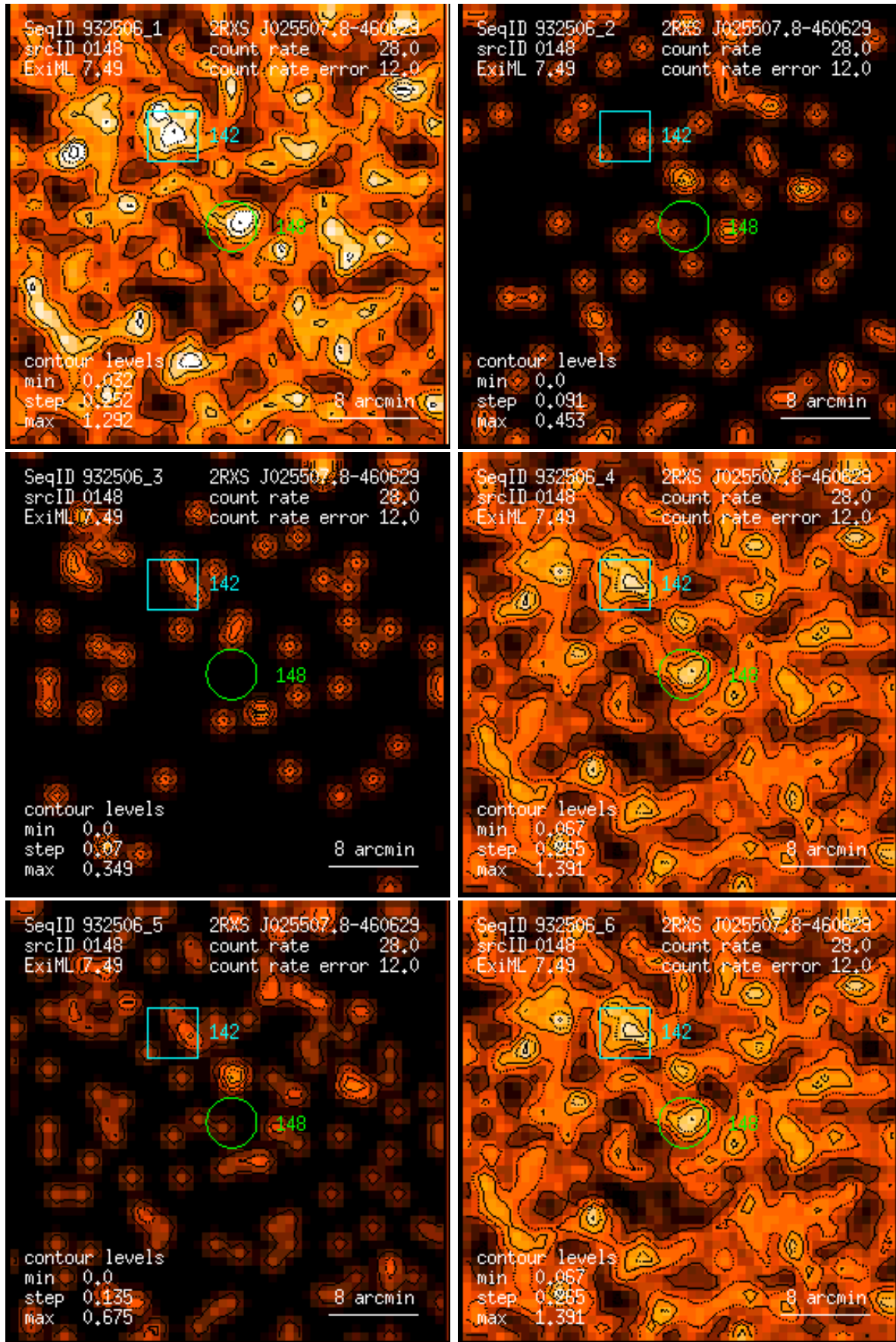
Figure 148: RASS 932506: detection 0148: band rate images, Gaussian filter: (1) PSPC channels 11 – 41, (2) 52 – 90, (3) 91 – 201, (4) 11 – 235, (5) 52 – 201, (6) 11 – 201. Broad band rates in counts/ks. Band rate contour levels in counts/ks/arcmin 2 .
