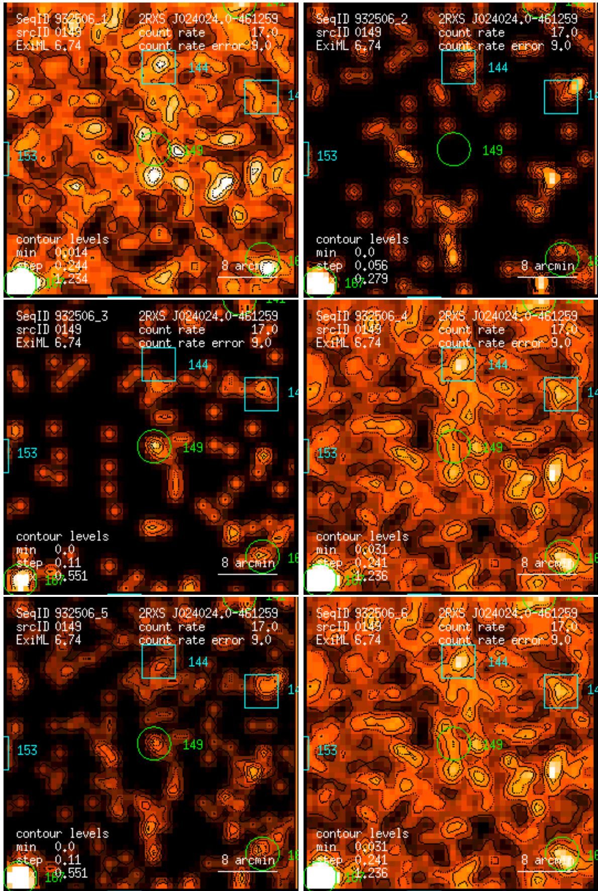
Figure 149: RASS 932506: detection 0149: band rate images, Gaussian filter: (1) PSPC channels 11 – 41, (2) 52 – 90, (3) 91 – 201, (4) 11 – 235, (5) 52 – 201, (6) 11 – 201. Broad band rates in counts/ks. Band rate contour levels in counts/ks/arcmin 2 .
