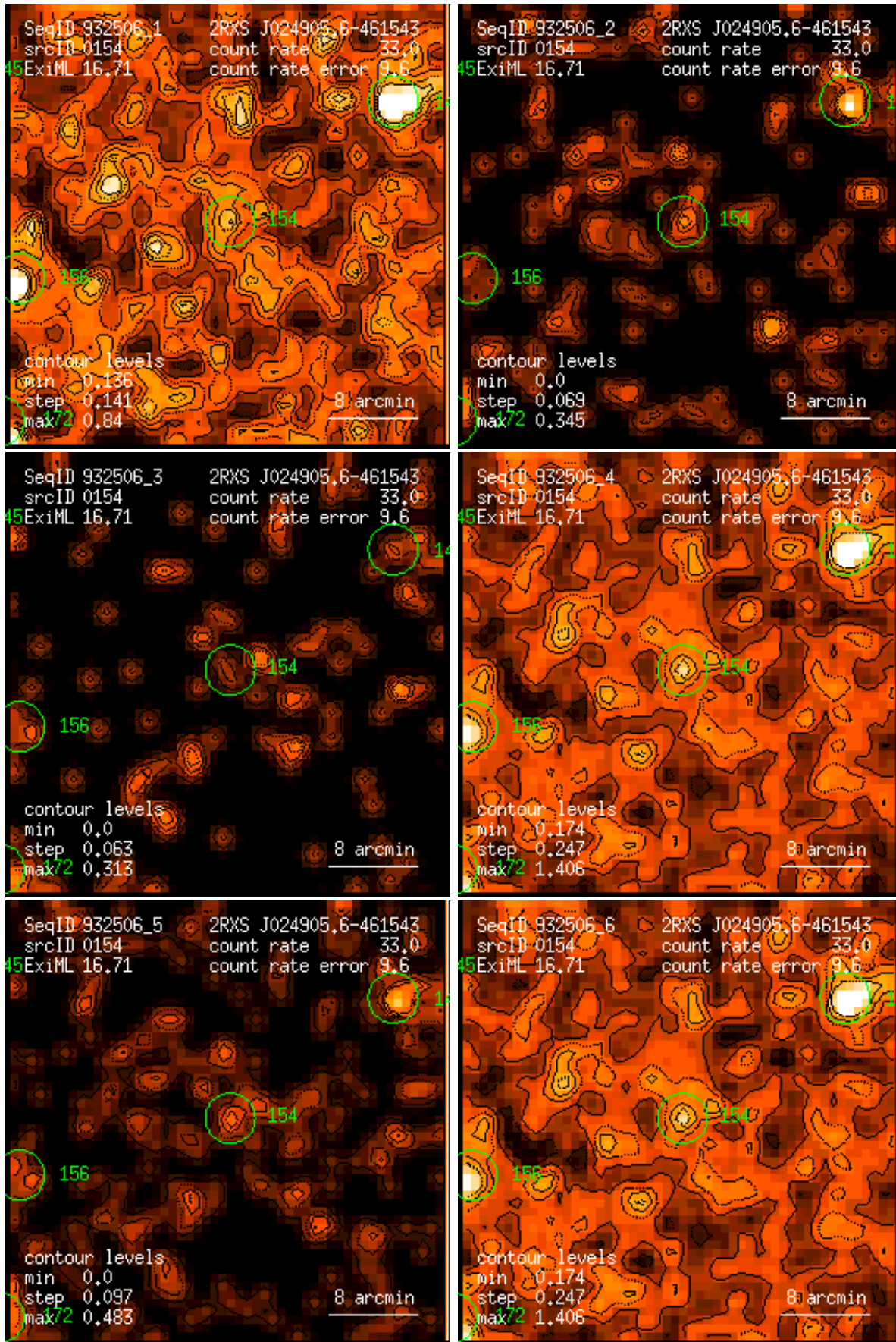
Figure 154: RASS 932506: detection 0154: band rate images, Gaussian filter: (1) PSPC channels 11 – 41, (2) 52 – 90, (3) 91 – 201, (4) 11 – 235, (5) 52 – 201, (6) 11 – 201. Broad band rates in counts/ks. Band rate contour levels in counts/ks/arcmin 2 .
