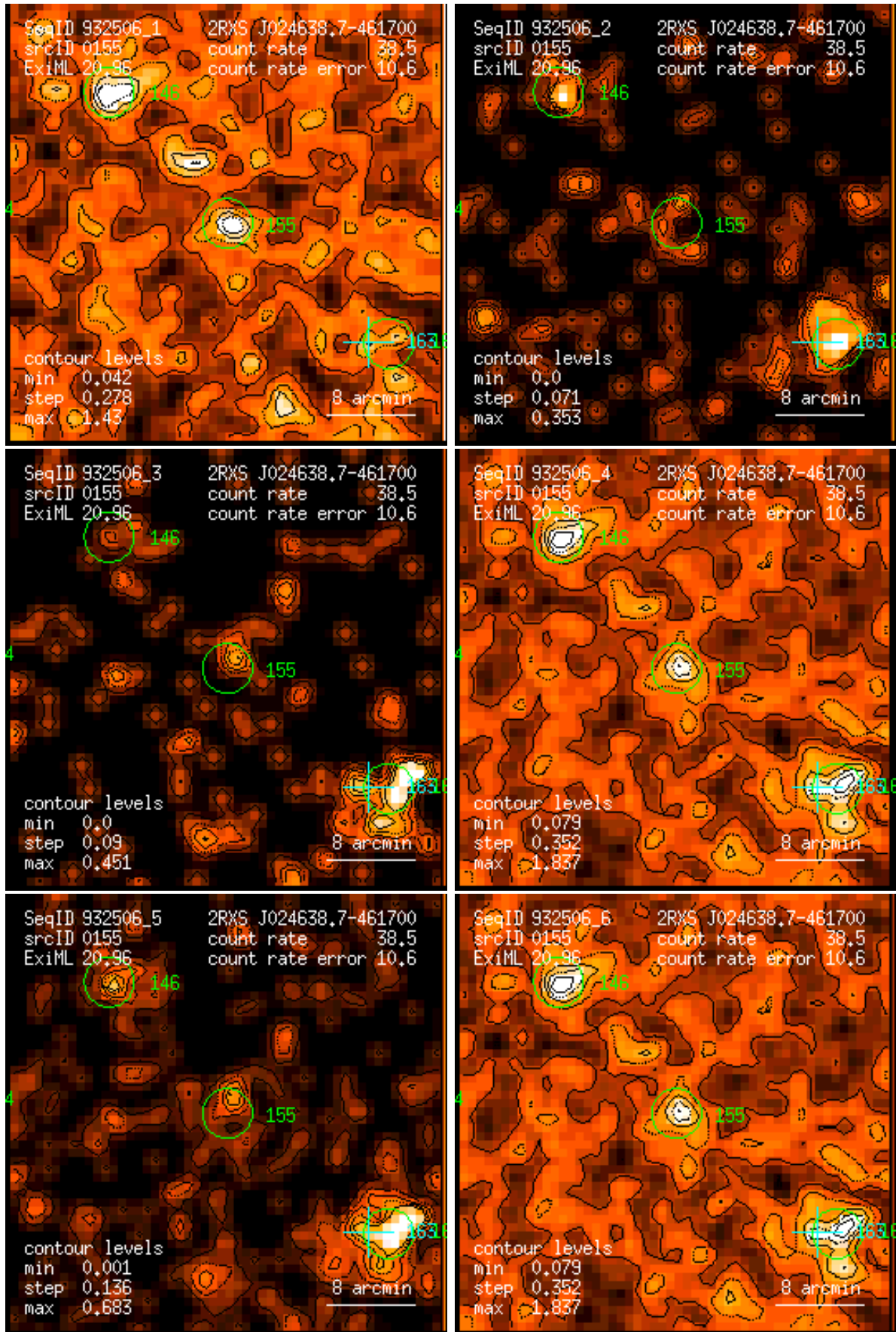
Figure 155: RASS 932506: detection 0155: band rate images, Gaussian filter: (1) PSPC channels 11 – 41, (2) 52 – 90, (3) 91 – 201, (4) 11 – 235, (5) 52 – 201, (6) 11 – 201. Broad band rates in counts/ks. Band rate contour levels in counts/ks/arcmin 2 .
