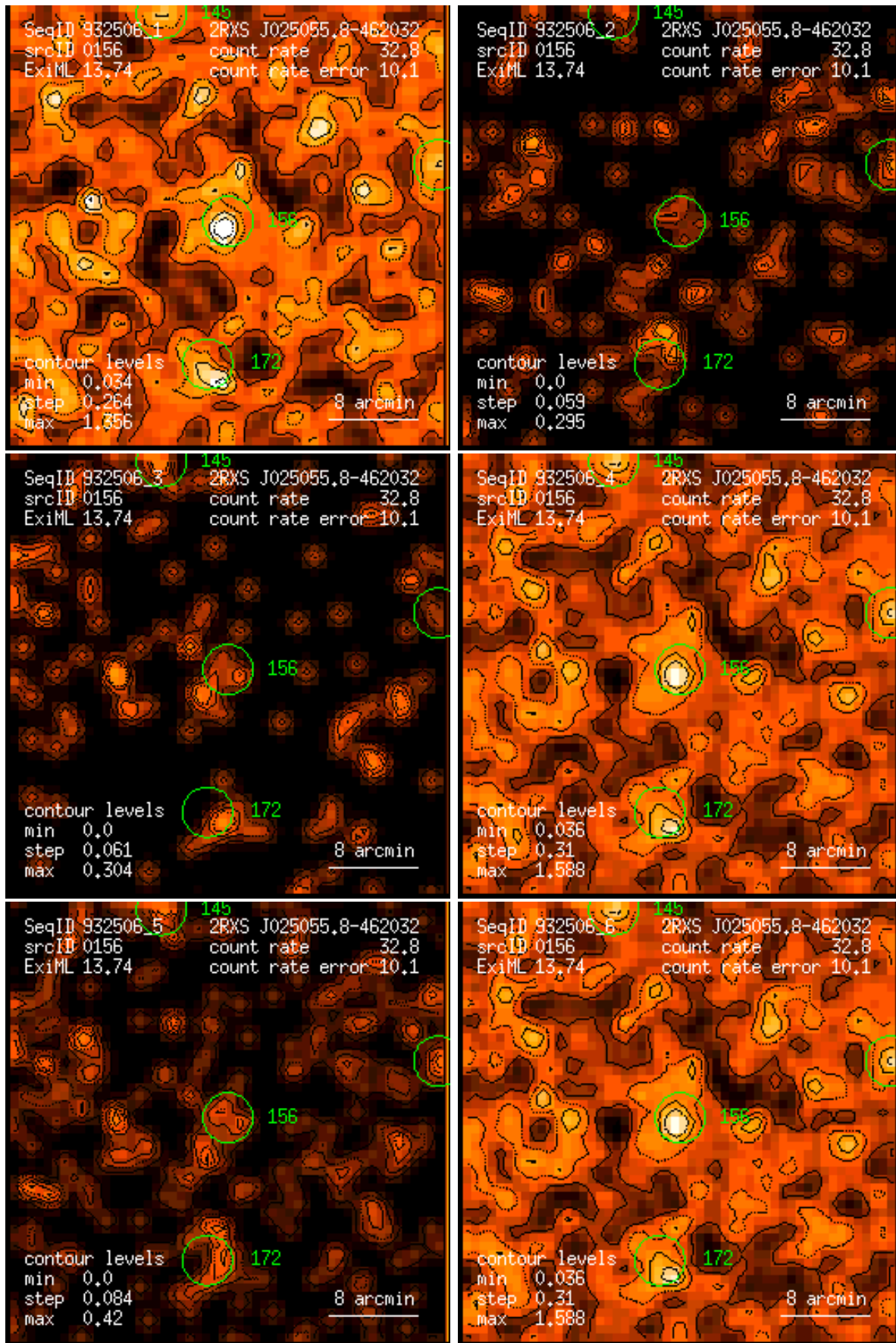
Figure 156: RASS 932506: detection 0156: band rate images, Gaussian filter: (1) PSPC channels 11 – 41, (2) 52 – 90, (3) 91 – 201, (4) 11 – 235, (5) 52 – 201, (6) 11 – 201. Broad band rates in counts/ks. Band rate contour levels in counts/ks/arcmin 2 .
