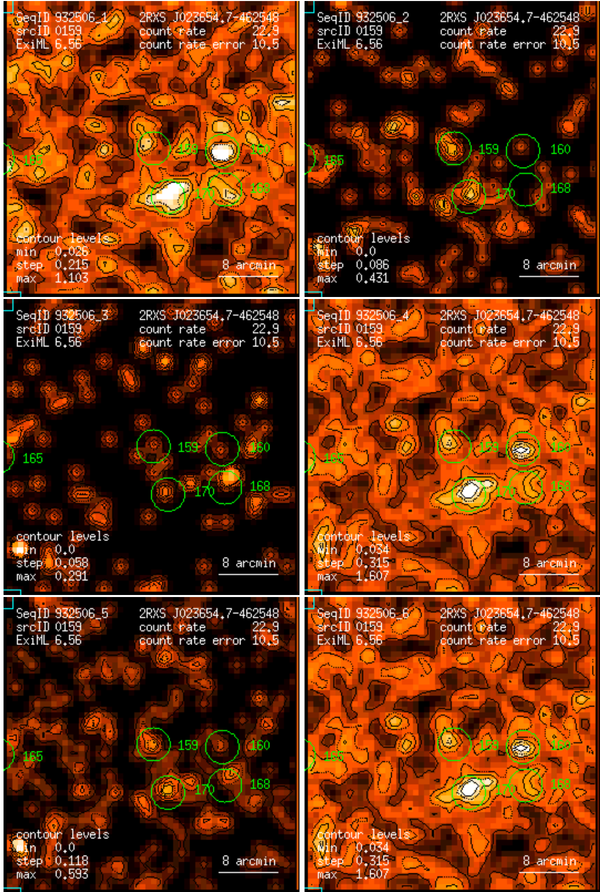
Figure 159: RASS 932506: detection 0159: band rate images, Gaussian filter: (1) PSPC channels 11 – 41, (2) 52 – 90, (3) 91 – 201, (4) 11 – 235, (5) 52 – 201, (6) 11 – 201. Broad band rates in counts/ks. Band rate contour levels in counts/ks/arcmin 2 .
