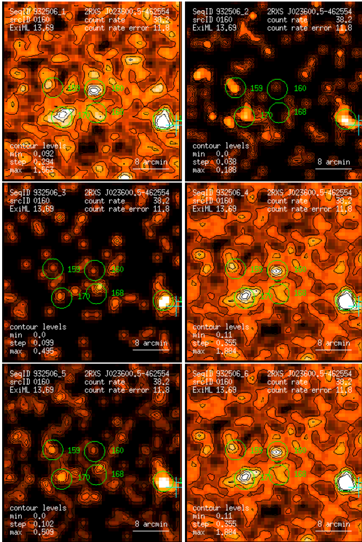
Figure 160: RASS 932506: detection 0160: band rate images, Gaussian filter: (1) PSPC channels 11 – 41, (2) 52 – 90, (3) 91 – 201, (4) 11 – 235, (5) 52 – 201, (6) 11 – 201. Broad band rates in counts/ks. Band rate contour levels in counts/ks/arcmin 2 .
