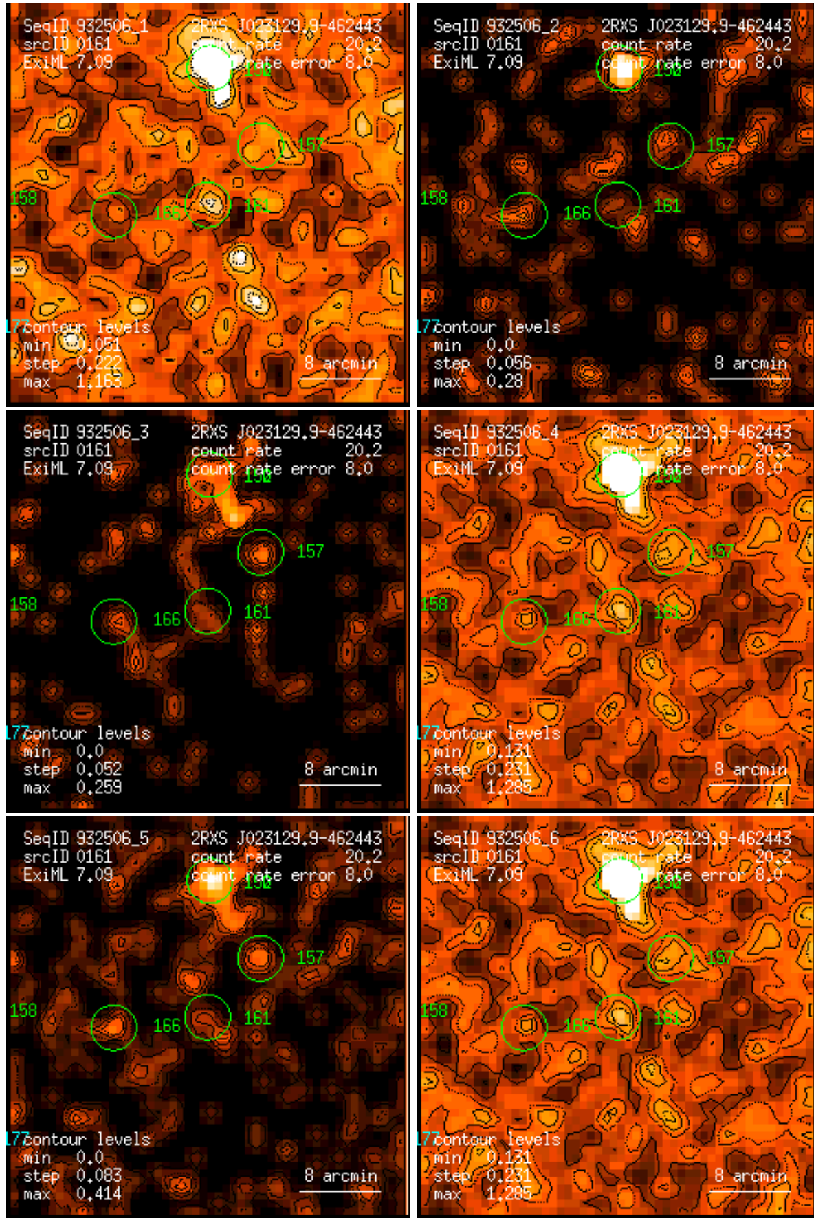
Figure 161: RASS 932506: detection 0161: band rate images, Gaussian filter: (1) PSPC channels 11 – 41, (2) 52 – 90, (3) 91 – 201, (4) 11 – 235, (5) 52 – 201, (6) 11 – 201. Broad band rates in counts/ks. Band rate contour levels in counts/ks/arcmin 2 .
