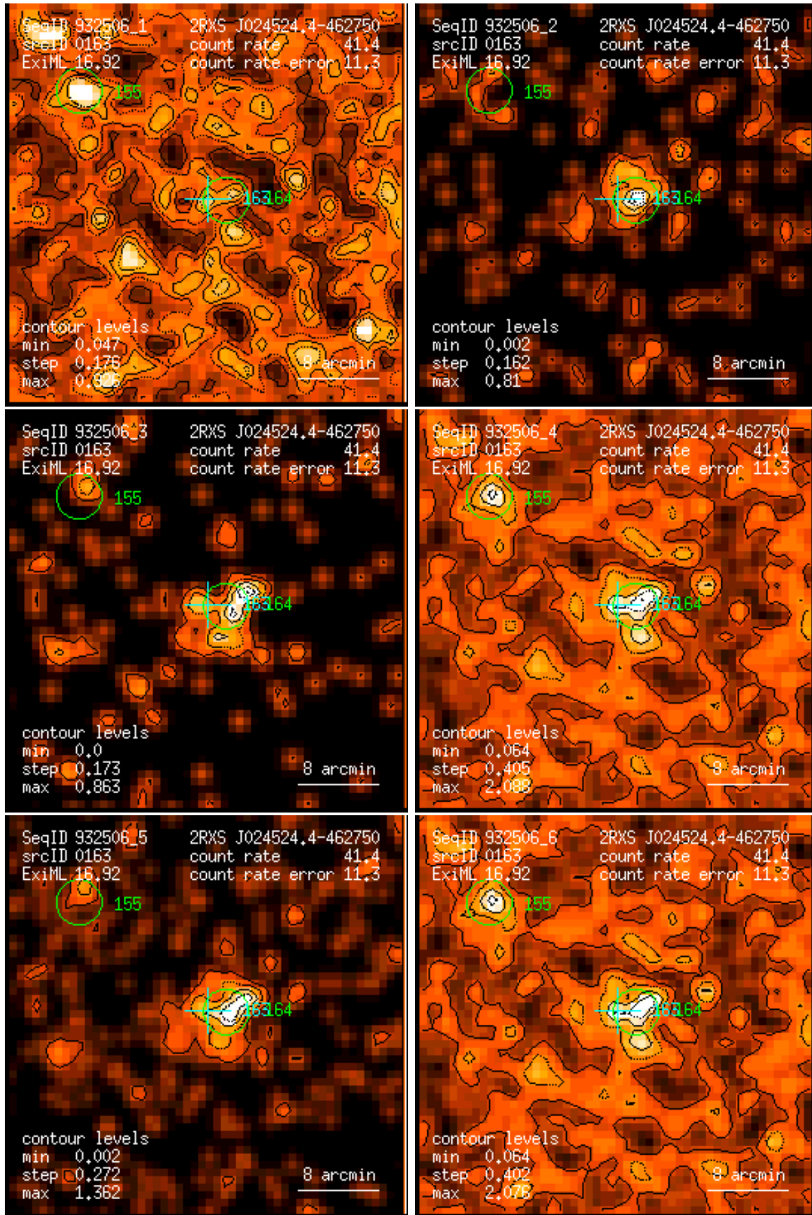
Figure 163: RASS 932506: detection 0163: band rate images, Gaussian filter: (1) PSPC channels 11 – 41, (2) 52 – 90, (3) 91 – 201, (4) 11 – 235, (5) 52 – 201, (6) 11 – 201. Broad band rates in counts/ks. Band rate contour levels in counts/ks/arcmin 2 .
