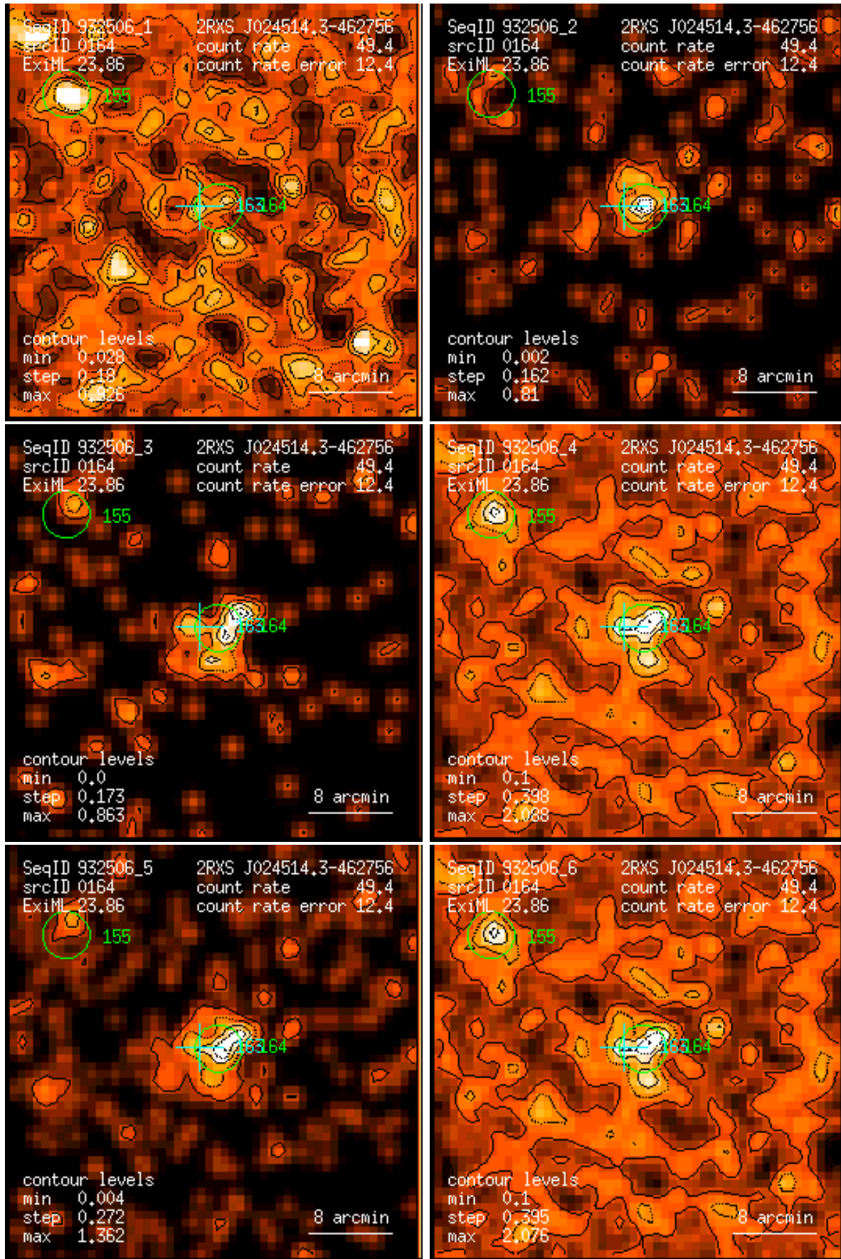
Figure 164: RASS 932506: detection 0164: band rate images, Gaussian filter: (1) PSPC channels 11 – 41, (2) 52 – 90, (3) 91 – 201, (4) 11 – 235, (5) 52 – 201, (6) 11 – 201. Broad band rates in counts/ks. Band rate contour levels in counts/ks/arcmin 2 .
