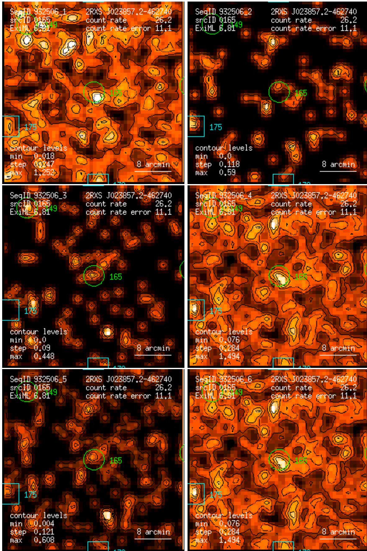
Figure 165: RASS 932506: detection 0165: band rate images, Gaussian filter: (1) PSPC channels 11 – 41, (2) 52 – 90, (3) 91 – 201, (4) 11 – 235, (5) 52 – 201, (6) 11 – 201. Broad band rates in counts/ks. Band rate contour levels in counts/ks/arcmin 2 .
