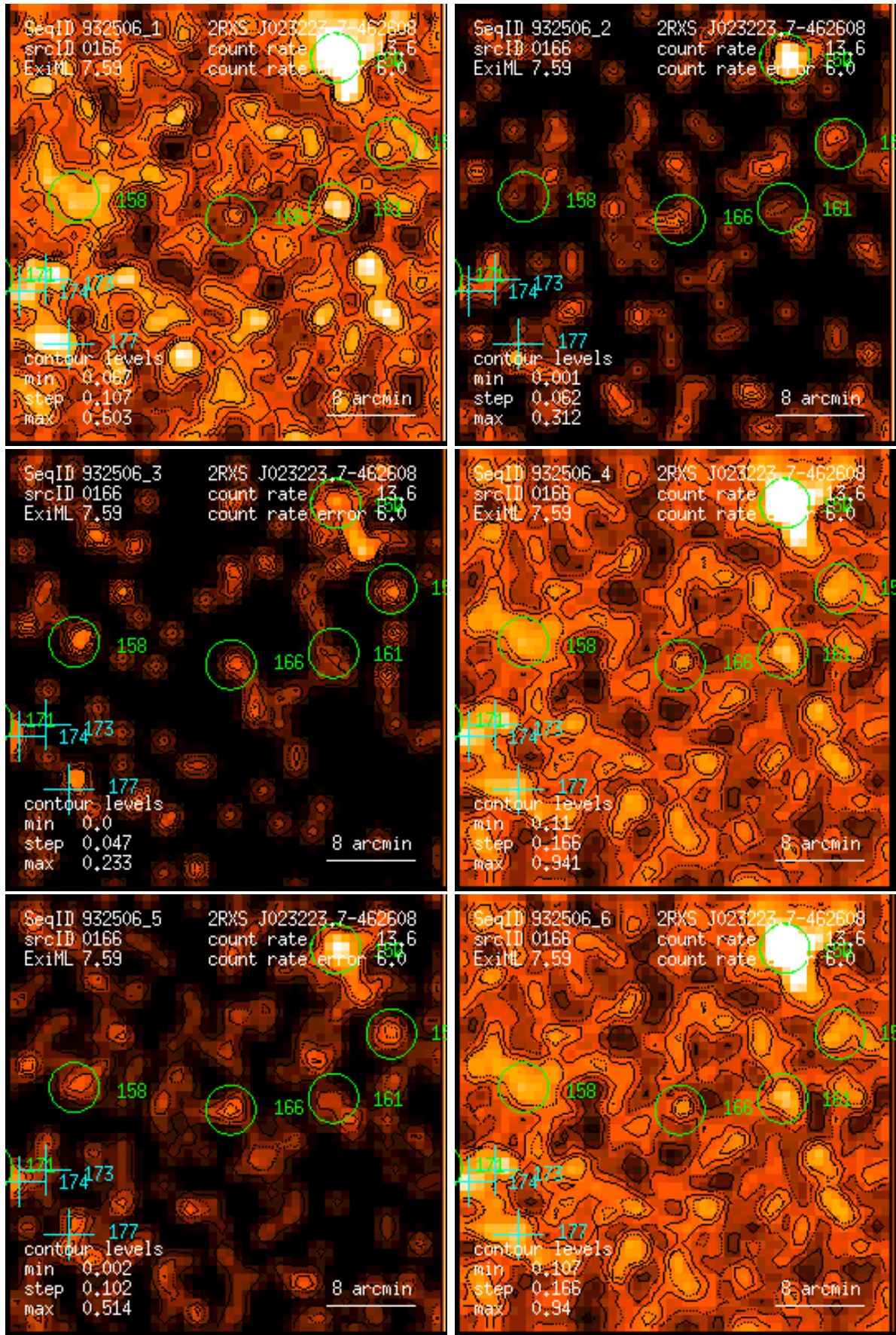
Figure 166: RASS 932506: detection 0166: band rate images, Gaussian filter: (1) PSPC channels 11 – 41, (2) 52 – 90, (3) 91 – 201, (4) 11 – 235, (5) 52 – 201, (6) 11 – 201. Broad band rates in counts/ks. Band rate contour levels in counts/ks/arcmin 2 .
