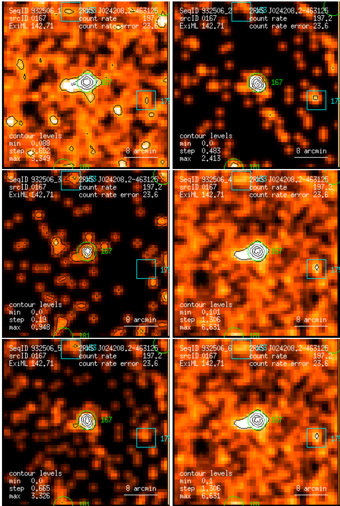
Figure 167: RASS 932506: detection 0167: band rate images, Gaussian filter: (1) PSPC channels 11 – 41, (2) 52 – 90, (3) 91 – 201, (4) 11 – 235, (5) 52 – 201, (6) 11 – 201. Broad band rates in counts/ks. Band rate contour levels in counts/ks/arcmin 2 .
