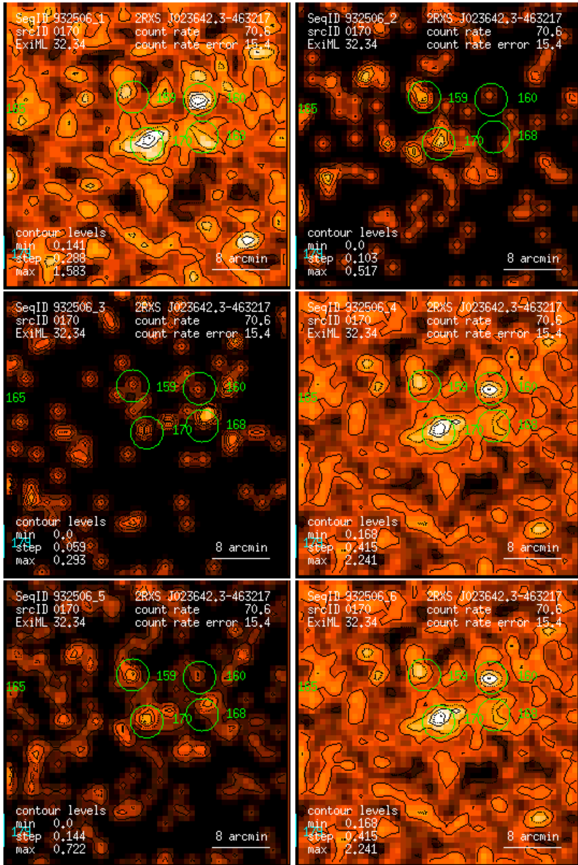
Figure 170: RASS 932506: detection 0170: band rate images, Gaussian filter: (1) PSPC channels 11 – 41, (2) 52 – 90, (3) 91 – 201, (4) 11 – 235, (5) 52 – 201, (6) 11 – 201. Broad band rates in counts/ks. Band rate contour levels in counts/ks/arcmin 2 .
