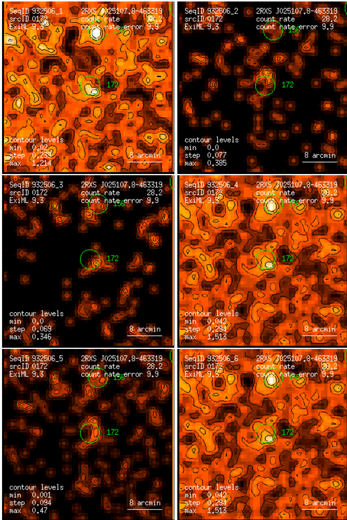
Figure 172: RASS 932506: detection 0172: band rate images, Gaussian filter: (1) PSPC channels 11 – 41, (2) 52 – 90, (3) 91 – 201, (4) 11 – 235, (5) 52 – 201, (6) 11 – 201. Broad band rates in counts/ks. Band rate contour levels in counts/ks/arcmin 2 .
