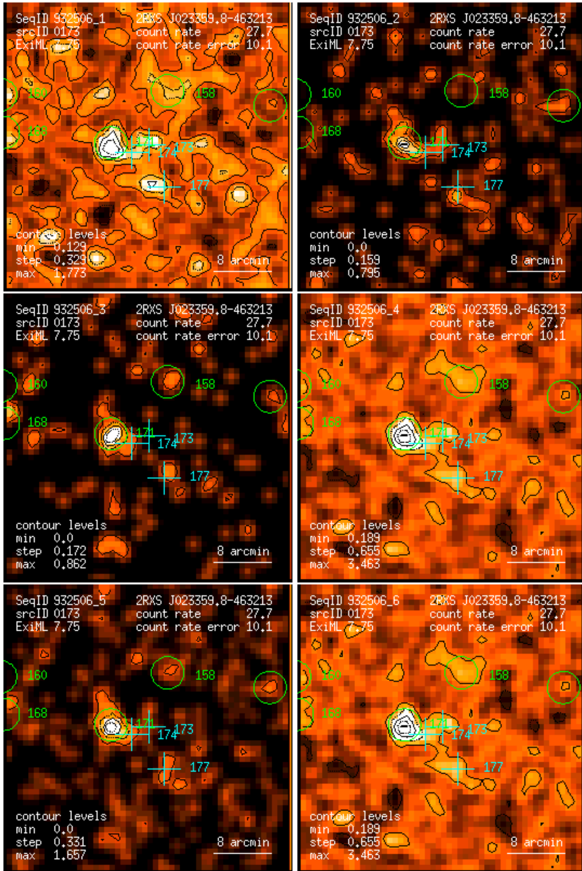
Figure 173: RASS 932506: detection 0173: band rate images, Gaussian filter: (1) PSPC channels 11 – 41, (2) 52 – 90, (3) 91 – 201, (4) 11 – 235, (5) 52 – 201, (6) 11 – 201. Broad band rates in counts/ks. Band rate contour levels in counts/ks/arcmin 2 .
