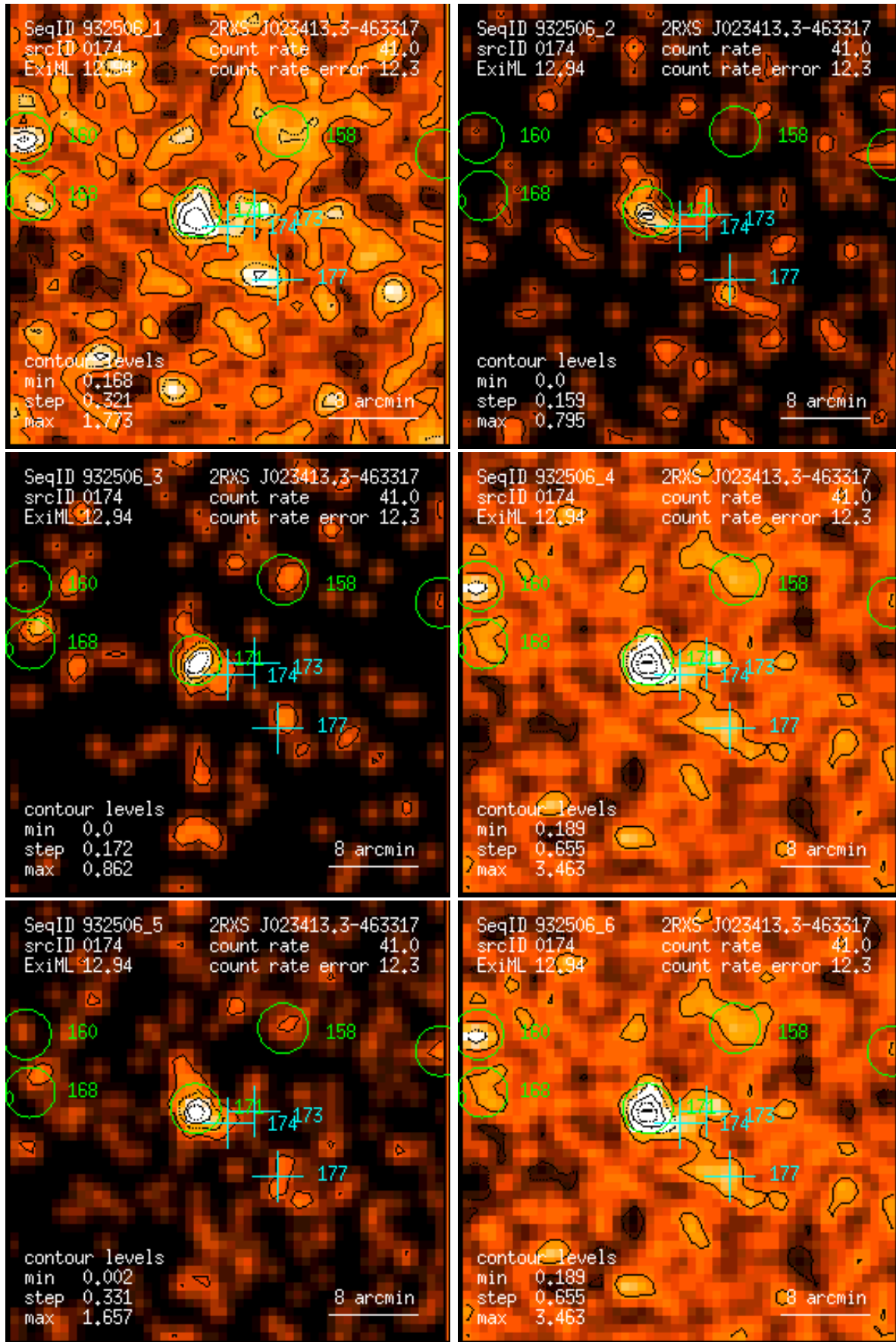
Figure 174: RASS 932506: detection 0174: band rate images, Gaussian filter: (1) PSPC channels 11 – 41, (2) 52 – 90, (3) 91 – 201, (4) 11 – 235, (5) 52 – 201, (6) 11 – 201. Broad band rates in counts/ks. Band rate contour levels in counts/ks/arcmin 2 .
