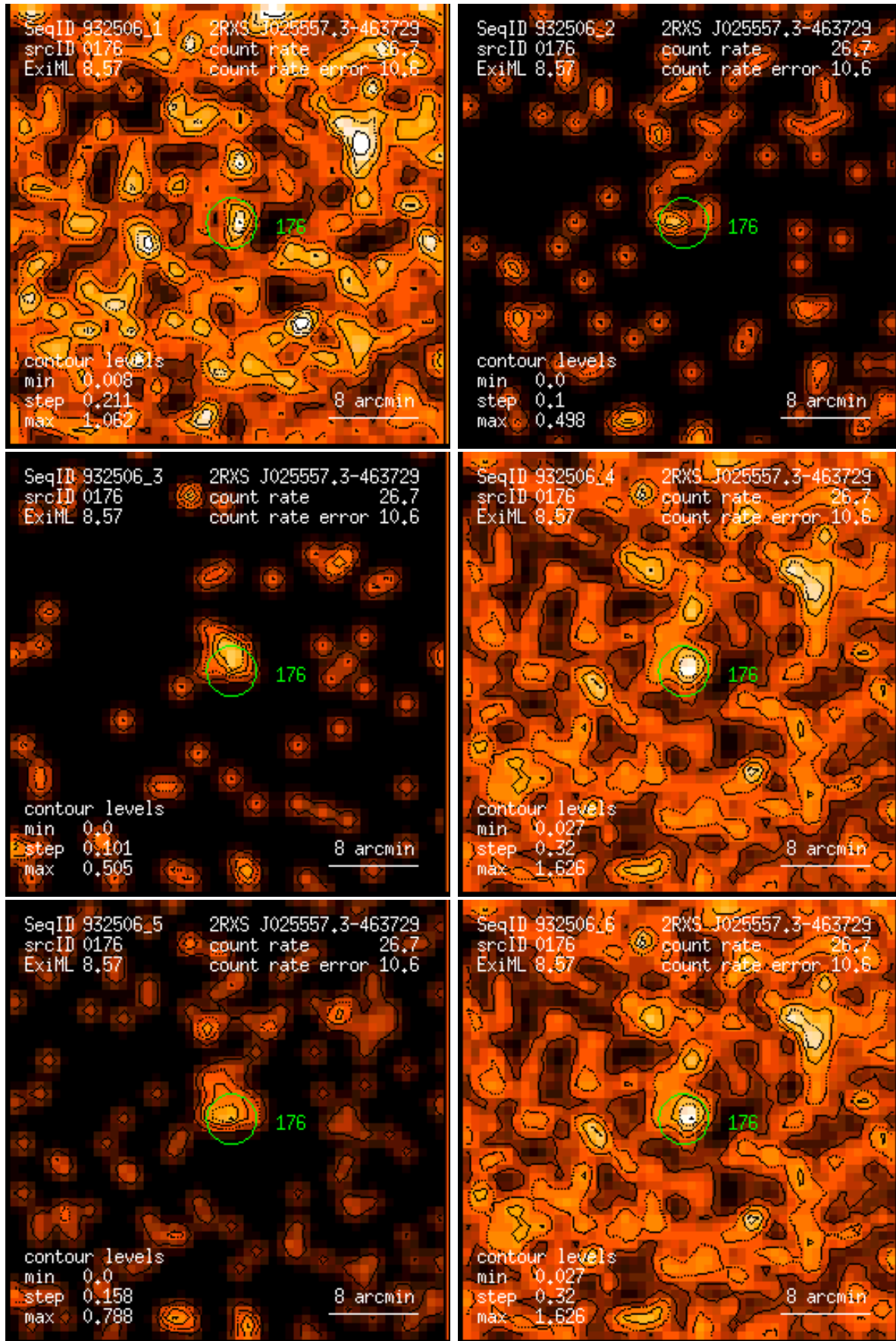
Figure 176: RASS 932506: detection 0176: band rate images, Gaussian filter: (1) PSPC channels 11 – 41, (2) 52 – 90, (3) 91 – 201, (4) 11 – 235, (5) 52 – 201, (6) 11 – 201. Broad band rates in counts/ks. Band rate contour levels in counts/ks/arcmin 2 .
