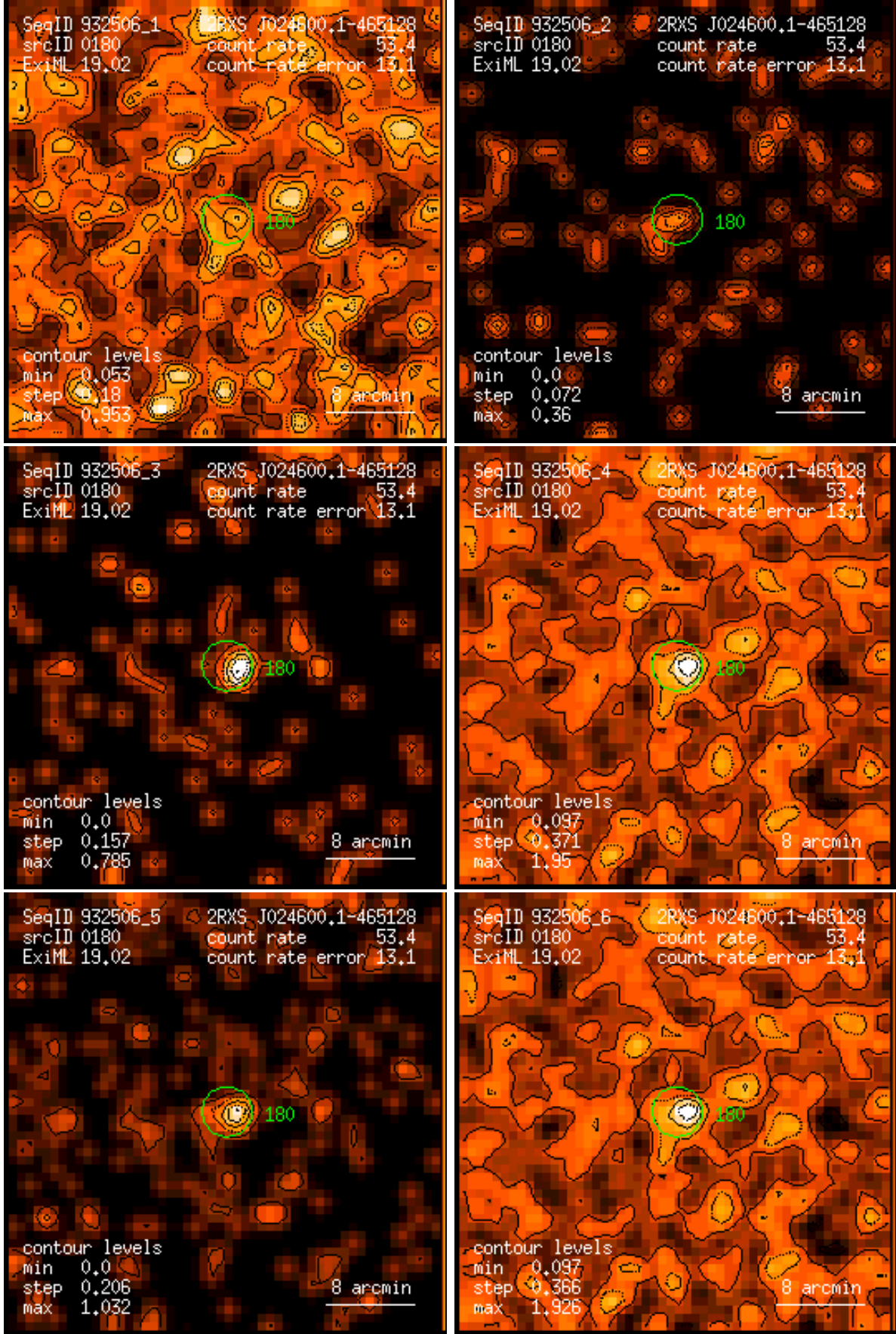
Figure 180: RASS 932506: detection 0180: band rate images, Gaussian filter: (1) PSPC channels 11 – 41, (2) 52 – 90, (3) 91 – 201, (4) 11 – 235, (5) 52 – 201, (6) 11 – 201. Broad band rates in counts/ks. Band rate contour levels in counts/ks/arcmin 2 .
