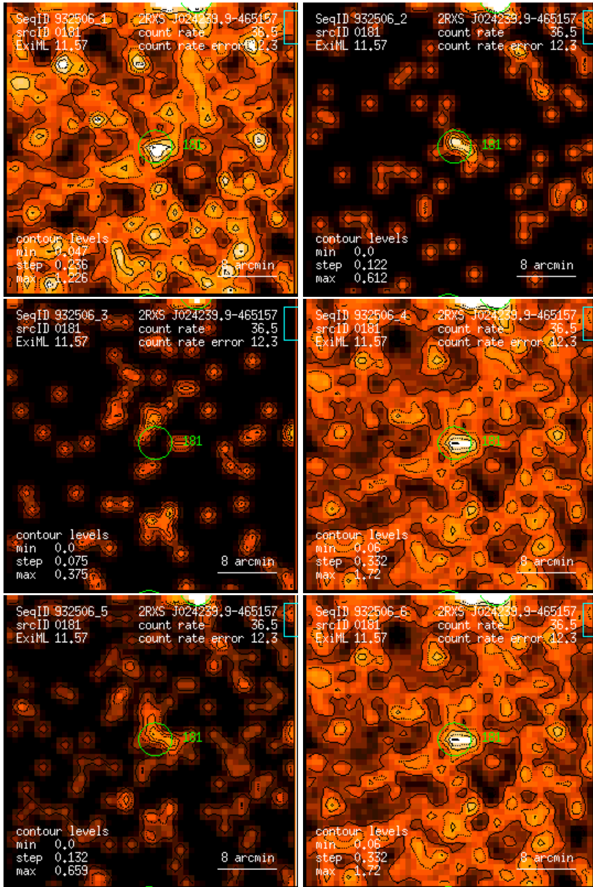
Figure 181: RASS 932506: detection 0181: band rate images, Gaussian filter: (1) PSPC channels 11 – 41, (2) 52 – 90, (3) 91 – 201, (4) 11 – 235, (5) 52 – 201, (6) 11 – 201. Broad band rates in counts/ks. Band rate contour levels in counts/ks/arcmin 2 .
