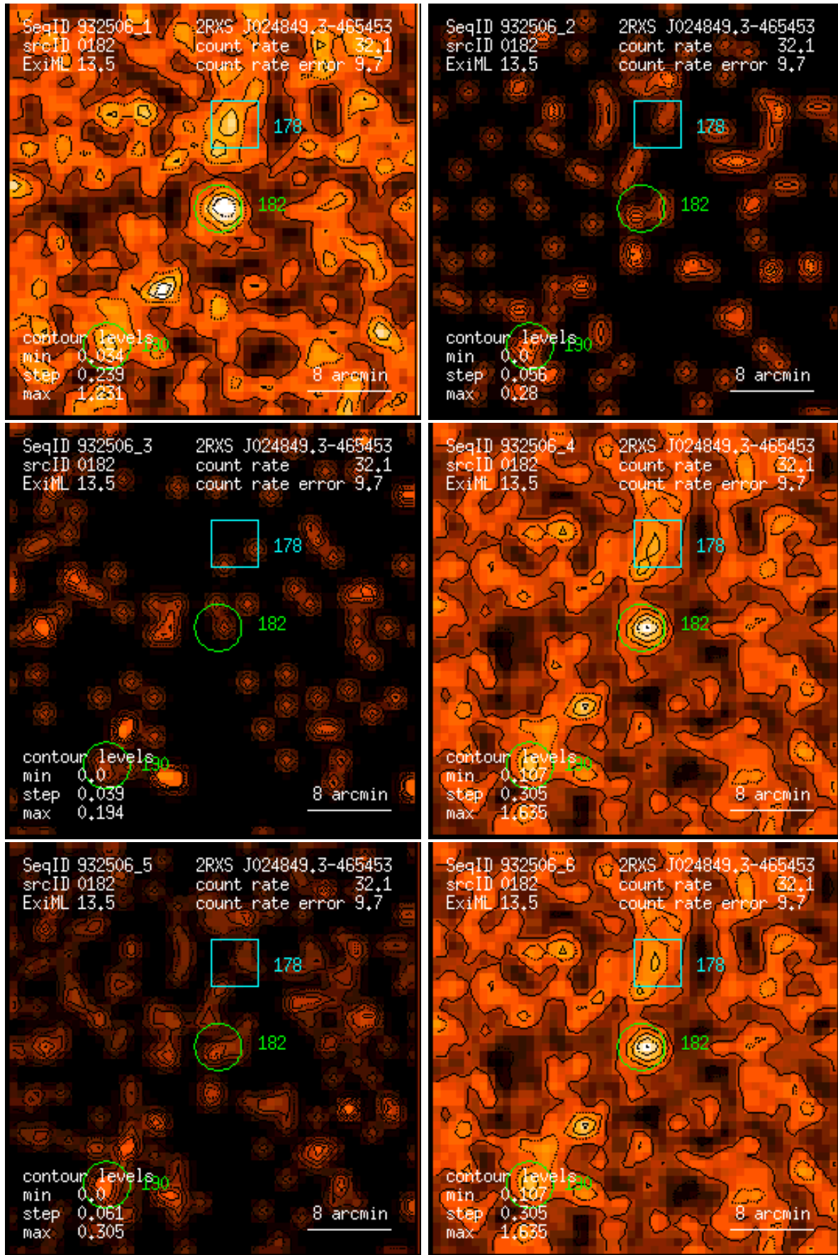
Figure 182: RASS 932506: detection 0182: band rate images, Gaussian filter: (1) PSPC channels 11 – 41, (2) 52 – 90, (3) 91 – 201, (4) 11 – 235, (5) 52 – 201, (6) 11 – 201. Broad band rates in counts/ks. Band rate contour levels in counts/ks/arcmin 2 .
