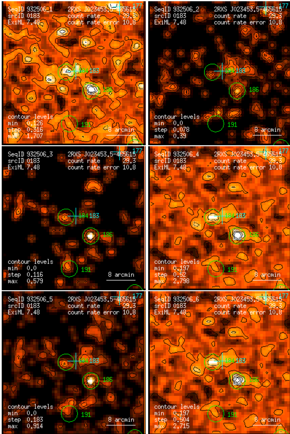
Figure 183: RASS 932506: detection 0183: band rate images, Gaussian filter: (1) PSPC channels 11 – 41, (2) 52 – 90, (3) 91 – 201, (4) 11 – 235, (5) 52 – 201, (6) 11 – 201. Broad band rates in counts/ks. Band rate contour levels in counts/ks/arcmin 2 .
