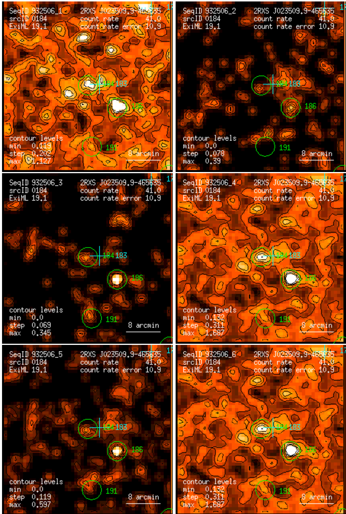
Figure 184: RASS 932506: detection 0184: band rate images, Gaussian filter: (1) PSPC channels 11 – 41, (2) 52 – 90, (3) 91 – 201, (4) 11 – 235, (5) 52 – 201, (6) 11 – 201. Broad band rates in counts/ks. Band rate contour levels in counts/ks/arcmin 2 .
