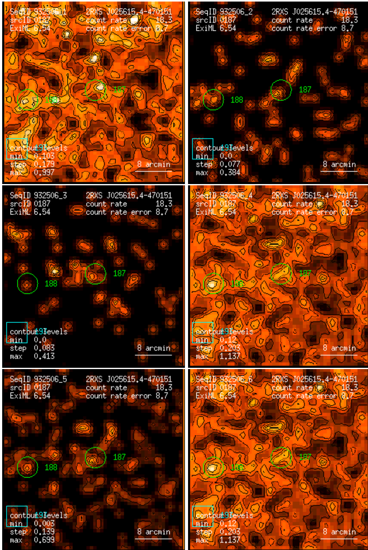
Figure 187: RASS 932506: detection 0187: band rate images, Gaussian filter: (1) PSPC channels 11 – 41, (2) 52 – 90, (3) 91 – 201, (4) 11 – 235, (5) 52 – 201, (6) 11 – 201. Broad band rates in counts/ks. Band rate contour levels in counts/ks/arcmin 2 .
