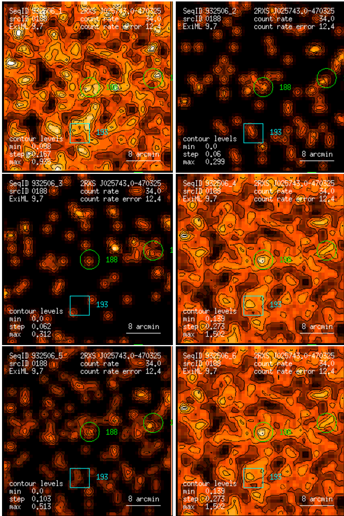
Figure 188: RASS 932506: detection 0188: band rate images, Gaussian filter: (1) PSPC channels 11 – 41, (2) 52 – 90, (3) 91 – 201, (4) 11 – 235, (5) 52 – 201, (6) 11 – 201. Broad band rates in counts/ks. Band rate contour levels in counts/ks/arcmin 2 .
