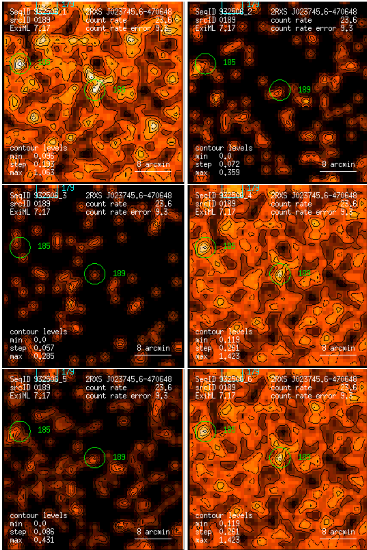
Figure 189: RASS 932506: detection 0189: band rate images, Gaussian filter: (1) PSPC channels 11 – 41, (2) 52 – 90, (3) 91 – 201, (4) 11 – 235, (5) 52 – 201, (6) 11 – 201. Broad band rates in counts/ks. Band rate contour levels in counts/ks/arcmin 2 .
