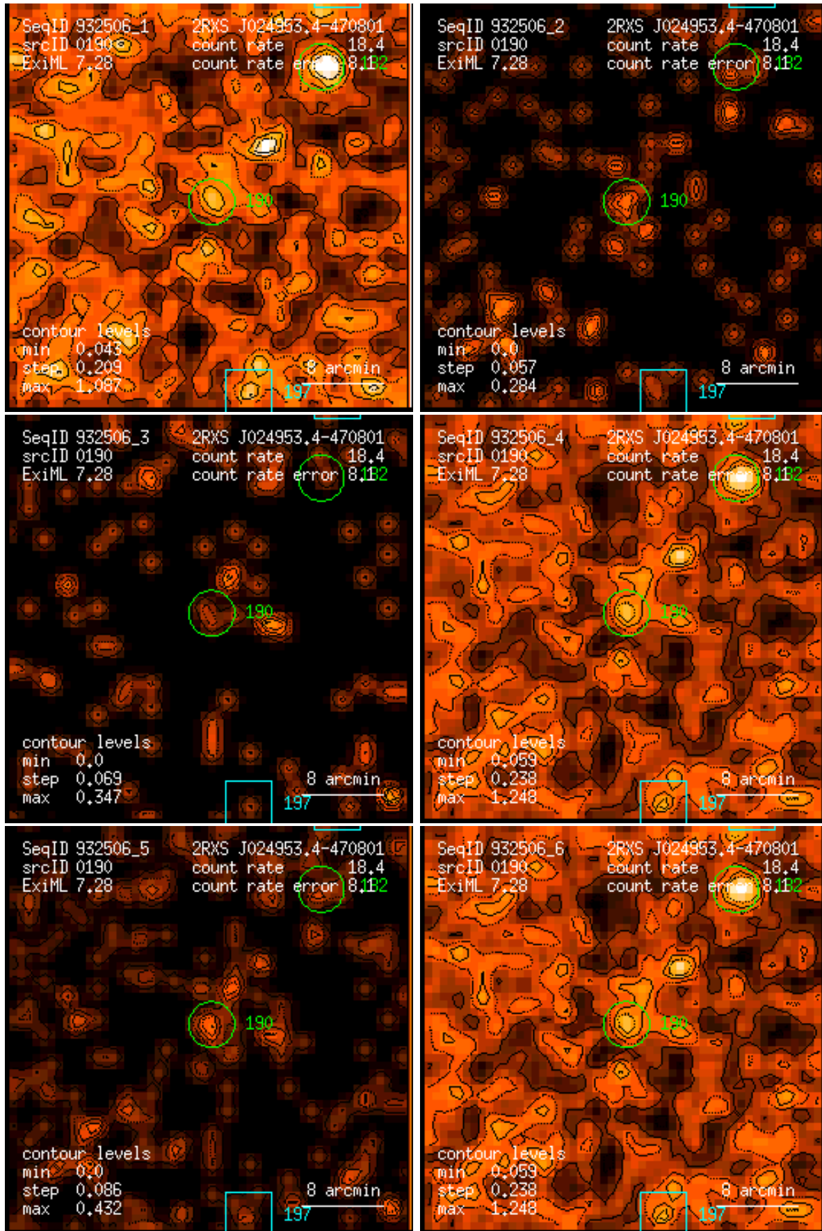
Figure 190: RASS 932506: detection 0190: band rate images, Gaussian filter: (1) PSPPC channels 11 – 41, (2) 52 – 90, (3) 91 – 201, (4) 11 – 235, (5) 52 – 201, (6) 11 – 201. Broad band rates in counts/ks. Band rate contour levels in counts/ks/arcmin 2 .
