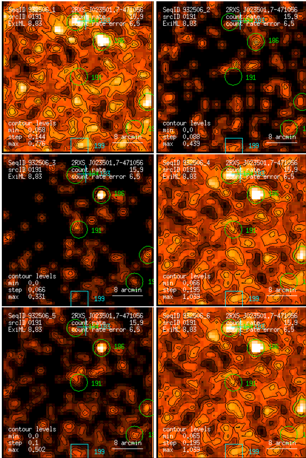
Figure 191: RASS 932506: detection 0191: band rate images, Gaussian filter: (1) PSPC channels 11 – 41, (2) 52 – 90, (3) 91 – 201, (4) 11 – 235, (5) 52 – 201, (6) 11 – 201. Broad band rates in counts/ks. Band rate contour levels in counts/ks/arcmin 2 .
