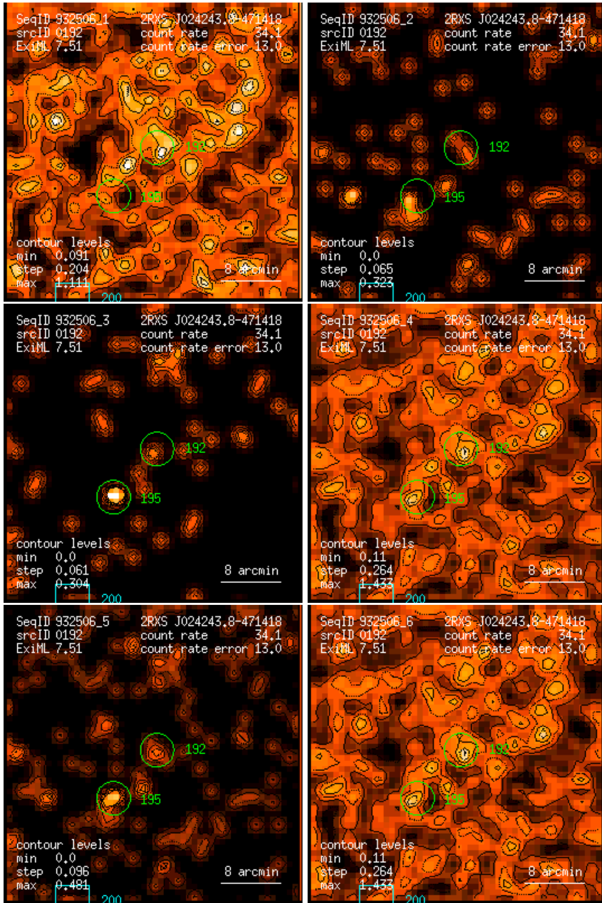
Figure 192: RASS 932506: detection 0192: band rate images, Gaussian filter: (1) PSPC channels 11 – 41, (2) 52 – 90, (3) 91 – 201, (4) 11 – 235, (5) 52 – 201, (6) 11 – 201. Broad band rates in counts/ks. Band rate contour levels in counts/ks/arcmin 2 .
