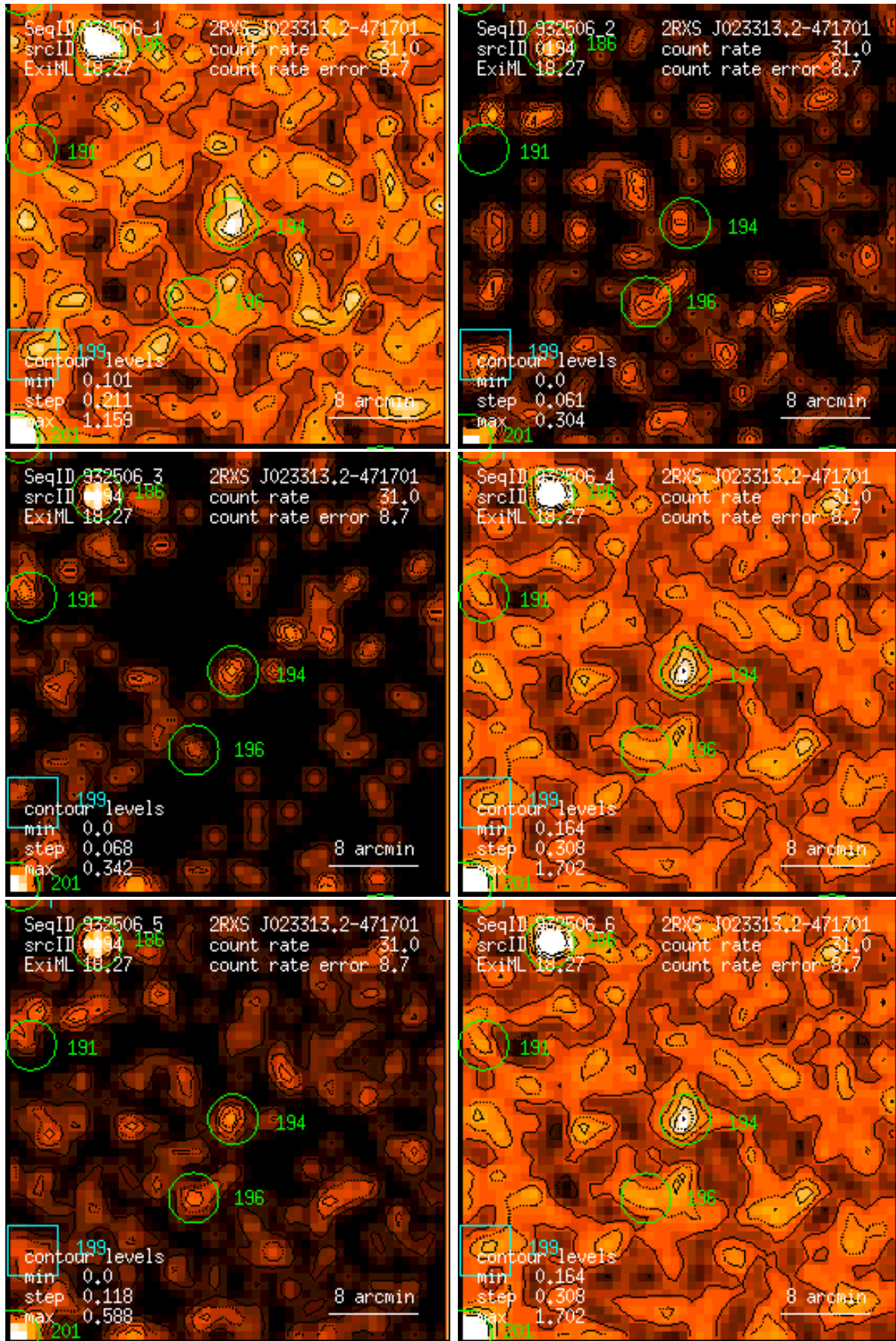
Figure 194: RASS 932506: detection 0194: band rate images, Gaussian filter: (1) PSPC channels 11 – 41, (2) 52 – 90, (3) 91 – 201, (4) 11 – 235, (5) 52 – 201, (6) 11 – 201. Broad band rates in counts/ks. Band rate contour levels in counts/ks/arcmin 2 .
