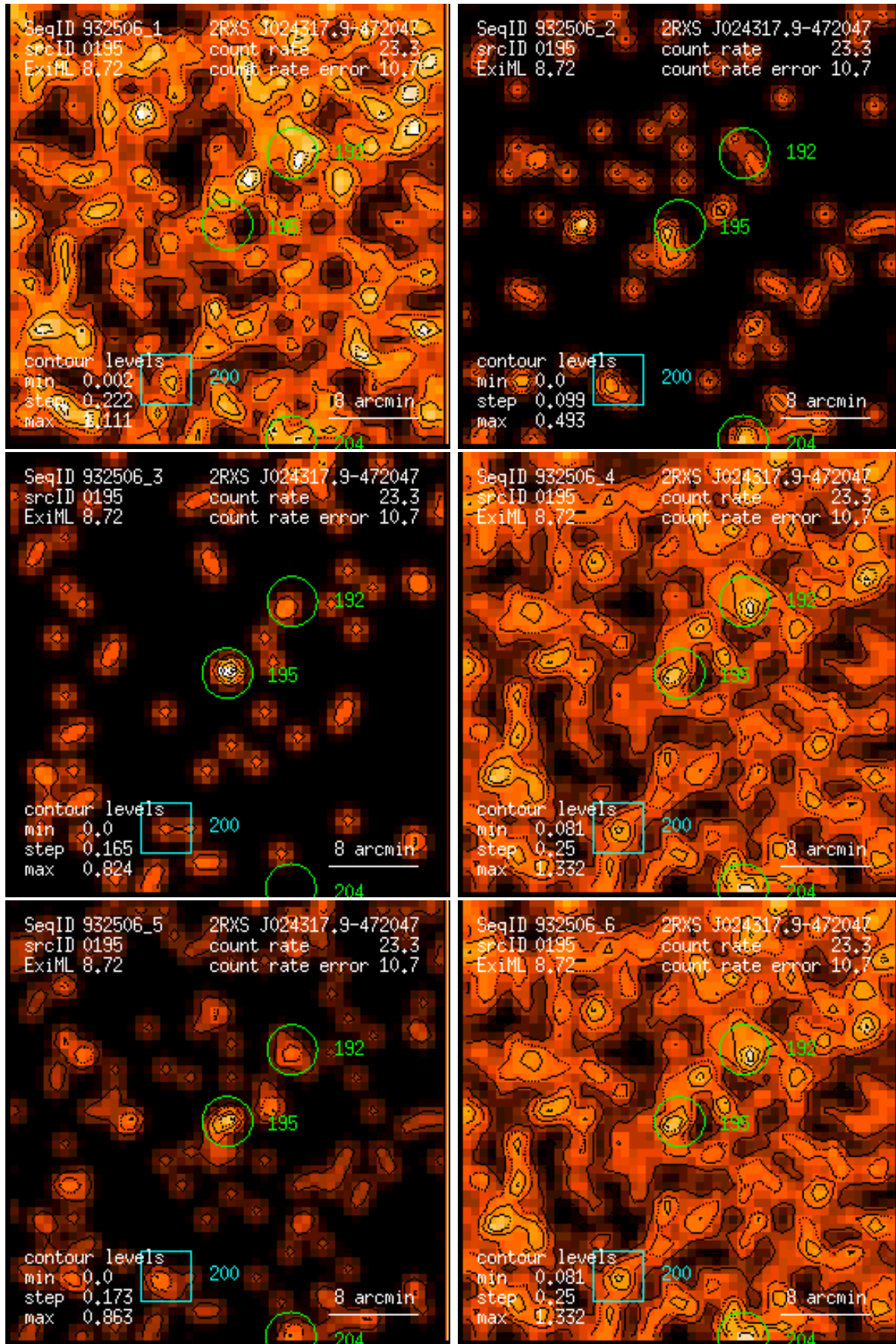
Figure 195: RASS 932506: detection 0195: band rate images, Gaussian filter: (1) PSPC channels 11 – 41, (2) 52 – 90, (3) 91 – 201, (4) 11 – 235, (5) 52 – 201, (6) 11 – 201. Broad band rates in counts/ks. Band rate contour levels in counts/ks/arcmin 2 .
