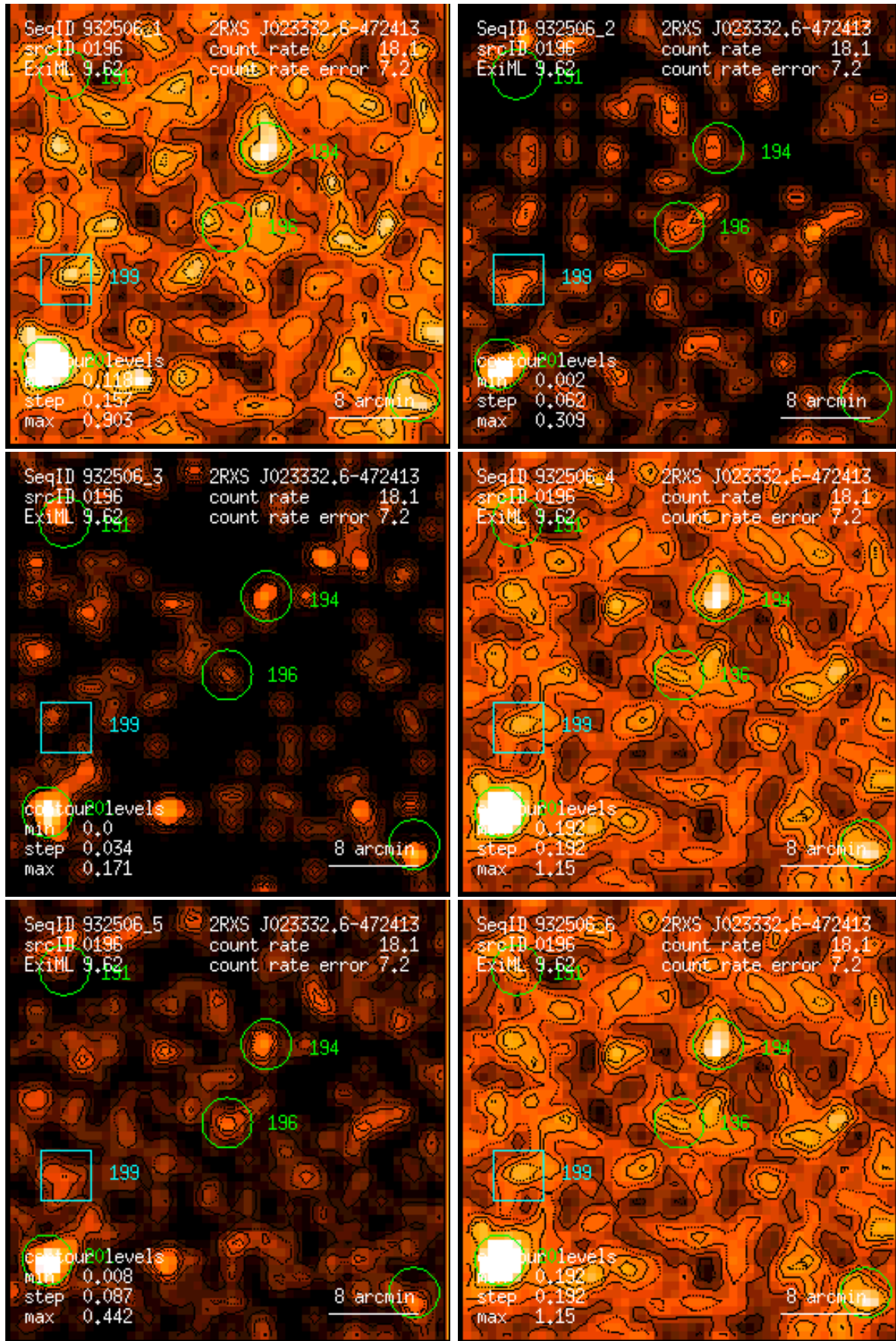
Figure 196: RASS 932506: detection 0196: band rate images, Gaussian filter: (1) PSPC channels 11 – 41, (2) 52 – 90, (3) 91 – 201, (4) 11 – 235, (5) 52 – 201, (6) 11 – 201. Broad band rates in counts/ks. Band rate contour levels in counts/ks/arcmin 2 .
