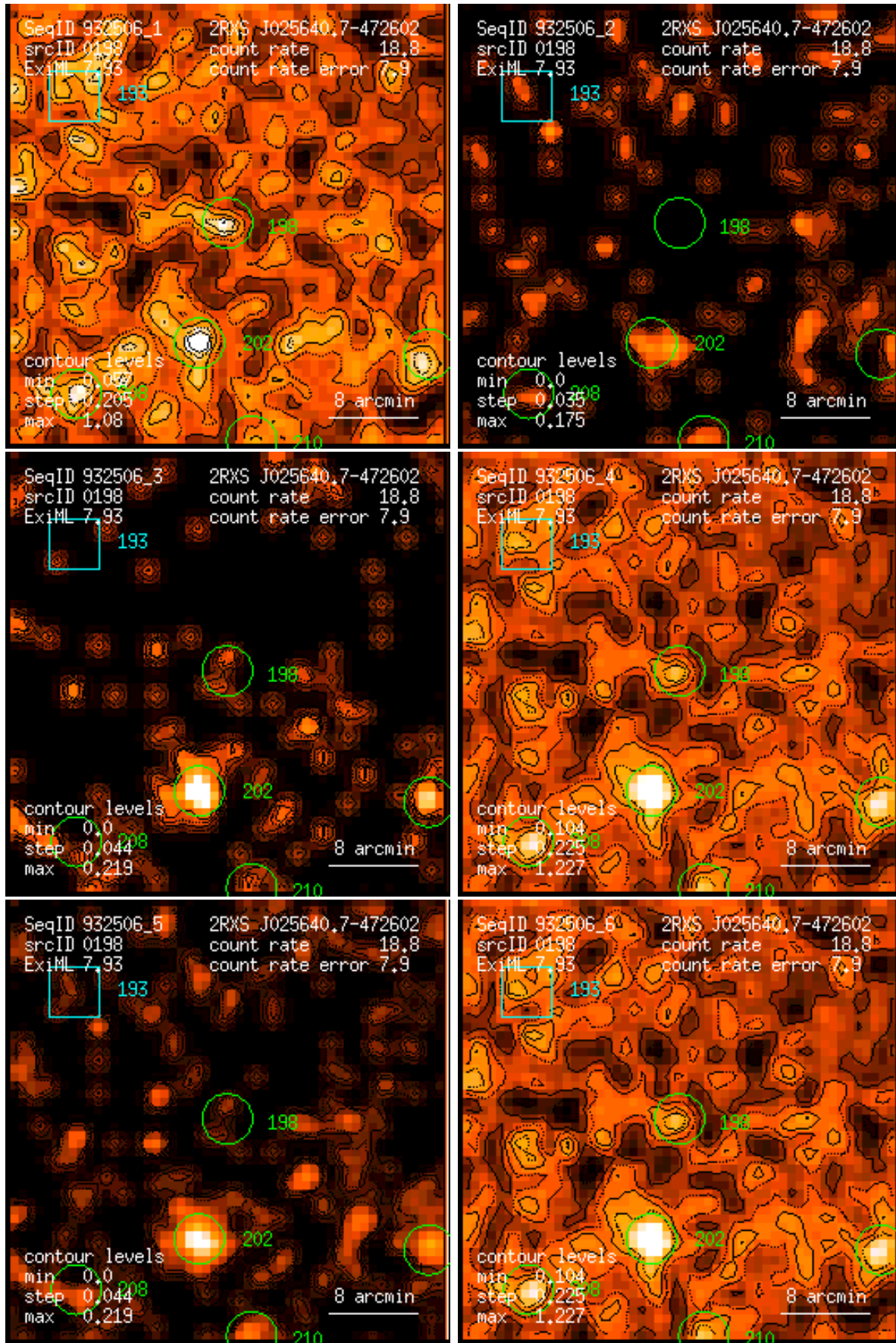
Figure 198: RASS 932506: detection 0198: band rate images, Gaussian filter: (1) PSPC channels 11 – 41, (2) 52 – 90, (3) 91 – 201, (4) 11 – 235, (5) 52 – 201, (6) 11 – 201. Broad band rates in counts/ks. Band rate contour levels in counts/ks/arcmin 2 .
