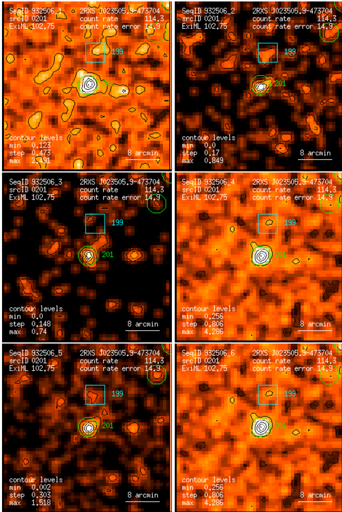
Figure 201: RASS 932506: detection 0201: band rate images, Gaussian filter: (1) PSPC channels 11 – 41, (2) 52 – 90, (3) 91 – 201, (4) 11 – 235, (5) 52 – 201, (6) 11 – 201. Broad band rates in counts/ks. Band rate contour levels in counts/ks/arcmin 2 .
