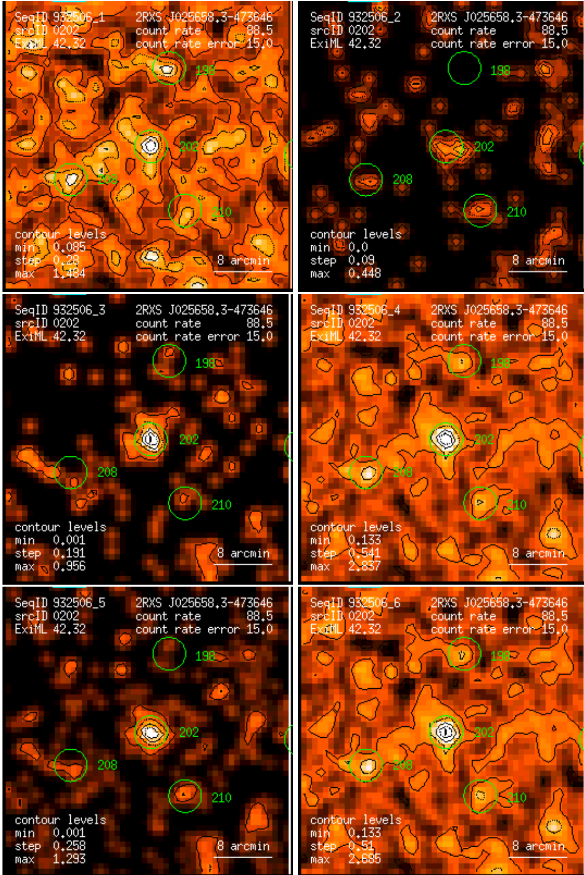
Figure 202: RASS 932506: detection 0202: band rate images, Gaussian filter: (1) PSPC channels 11 – 41, (2) 52 – 90, (3) 91 – 201, (4) 11 – 235, (5) 52 – 201, (6) 11 – 201. Broad band rates in counts/ks. Band rate contour levels in counts/ks/arcmin 2 .
