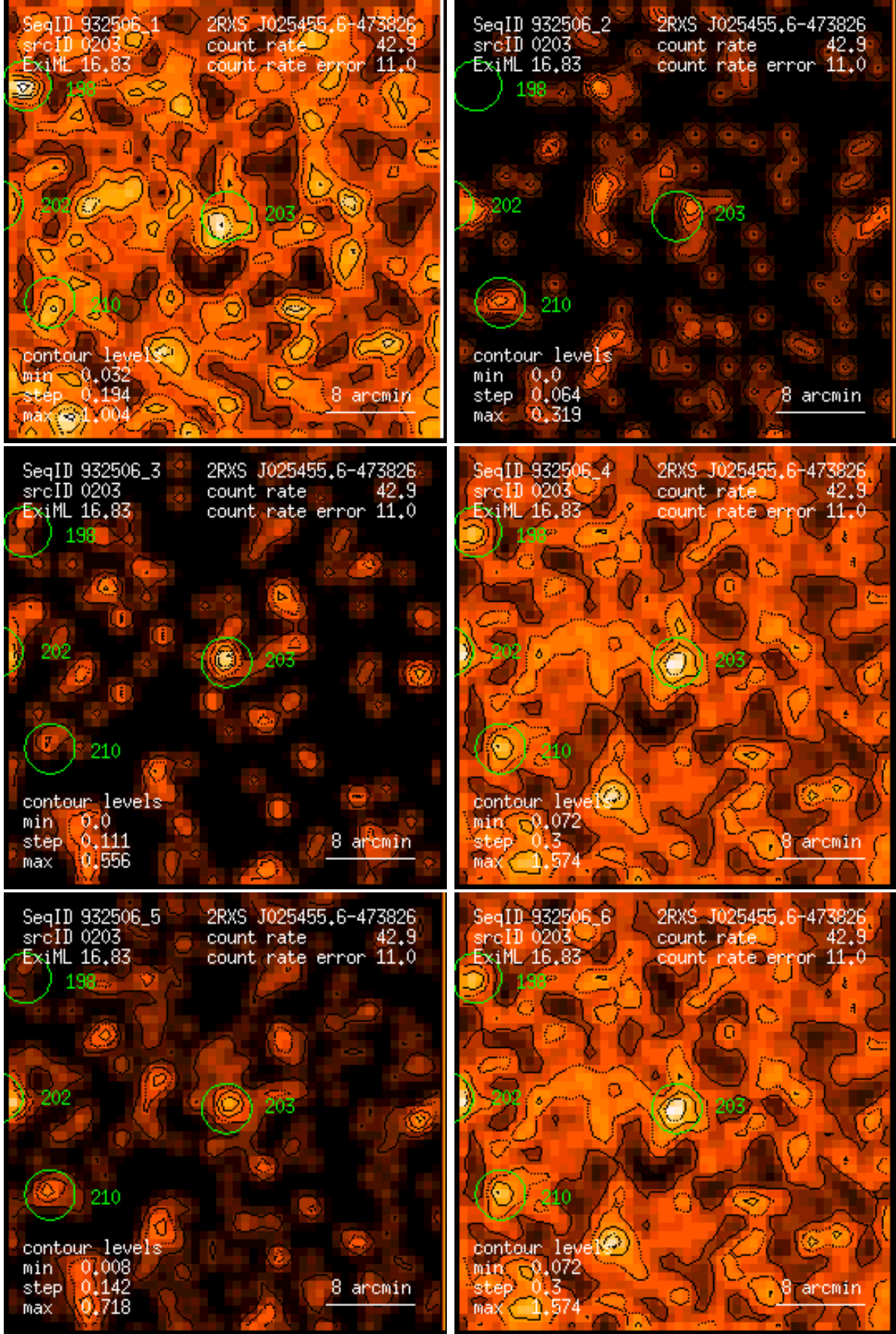
Figure 203: RASS 932506: detection 0203: band rate images, Gaussian filter: (1) PSPC channels 11 – 41, (2) 52 – 90, (3) 91 – 201, (4) 11 – 235, (5) 52 – 201, (6) 11 – 201. Broad band rates in counts/ks. Band rate contour levels in counts/ks/arcmin 2 .
