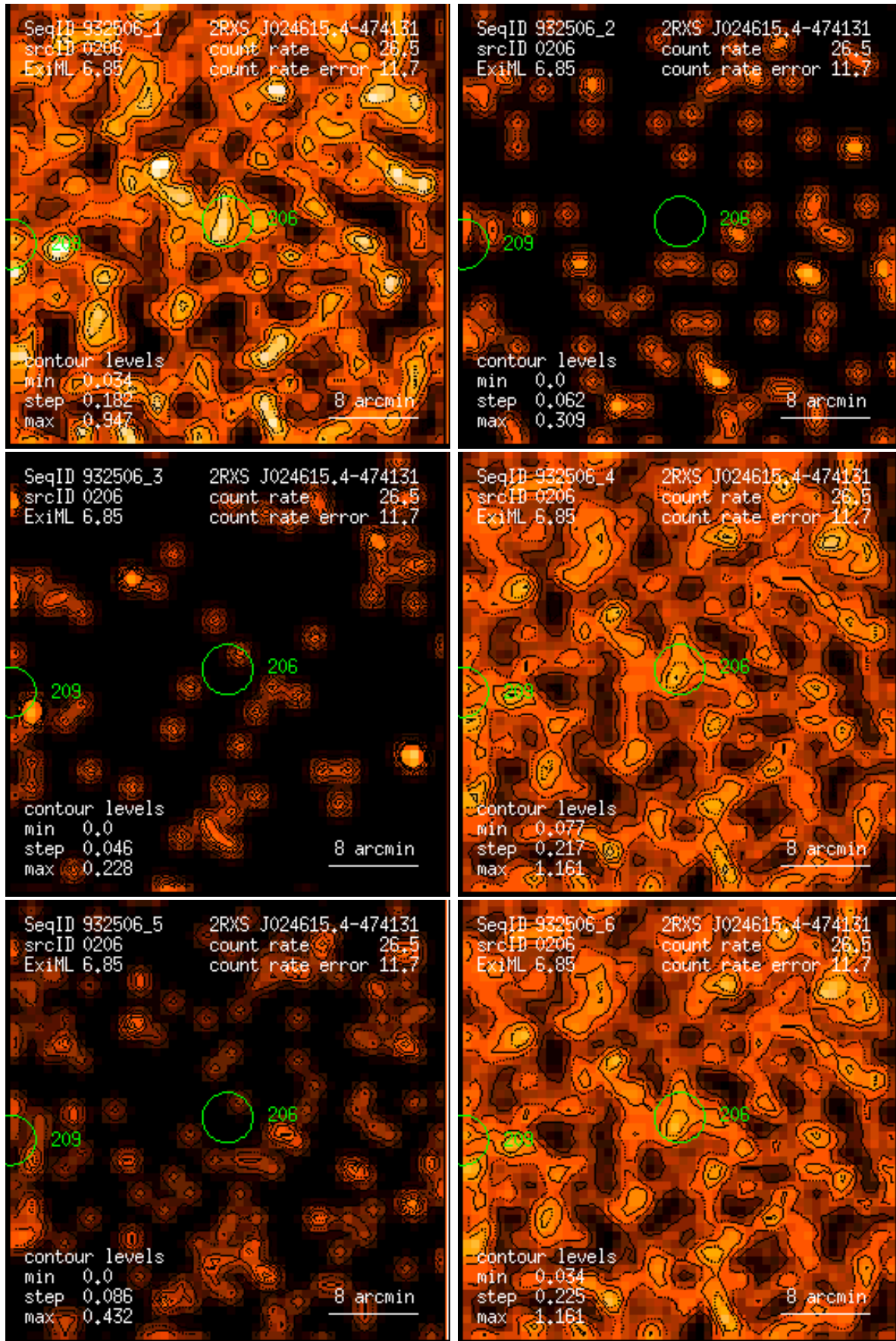
Figure 206: RASS 932506: detection 0206: band rate images, Gaussian filter: (1) PSPC channels 11 – 41, (2) 52 – 90, (3) 91 – 201, (4) 11 – 235, (5) 52 – 201, (6) 11 – 201. Broad band rates in counts/ks. Band rate contour levels in counts/ks/arcmin 2 .
