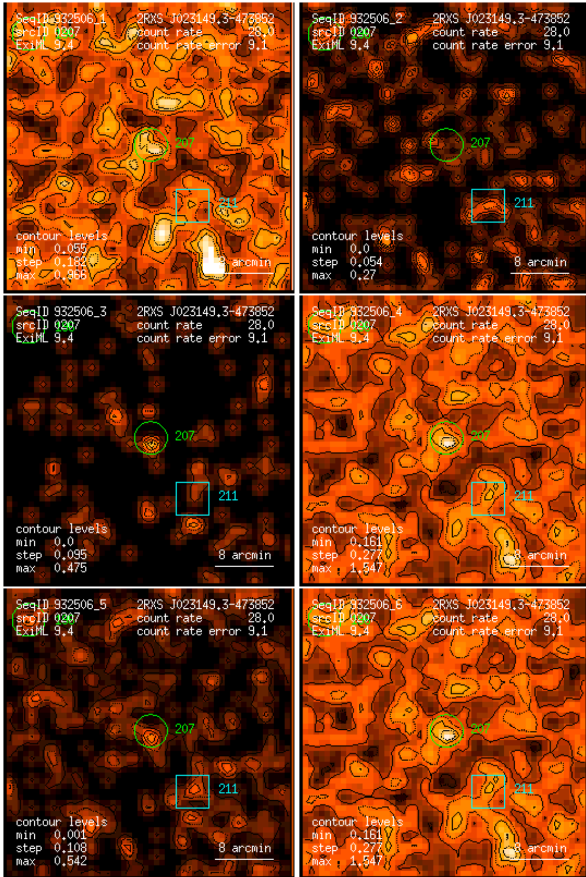
Figure 207: RASS 932506: detection 0207: band rate images, Gaussian filter: (1) PSPC channels 11 – 41, (2) 52 – 90, (3) 91 – 201, (4) 11 – 235, (5) 52 – 201, (6) 11 – 201. Broad band rates in counts/ks. Band rate contour levels in counts/ks/arcmin 2 .
