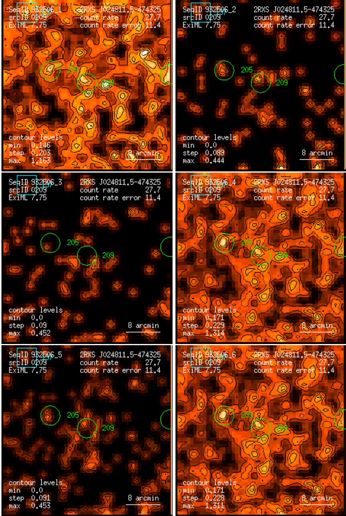
Figure 209: RASS 932506: detection 0209: band rate images, Gaussian filter: (1) PSPC channels 11 – 41, (2) 52 – 90, (3) 91 – 201, (4) 11 – 235, (5) 52 – 201, (6) 11 – 201. Broad band rates in counts/ks. Band rate contour levels in counts/ks/arcmin 2 .
