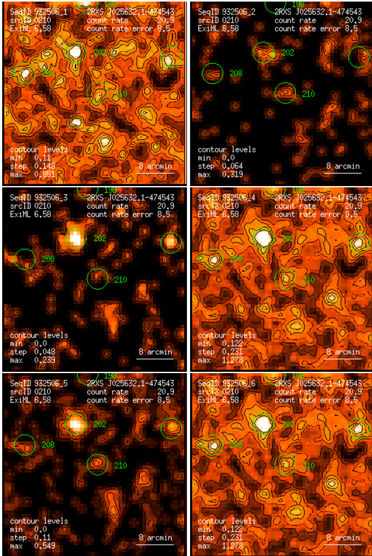
Figure 210: RASS 932506: detection 0210: band rate images, Gaussian filter: (1) PSPC channels 11 – 41, (2) 52 – 90, (3) 91 – 201, (4) 11 – 235, (5) 52 – 201, (6) 11 – 201. Broad band rates in counts/ks. Band rate contour levels in counts/ks/arcmin 2 .
