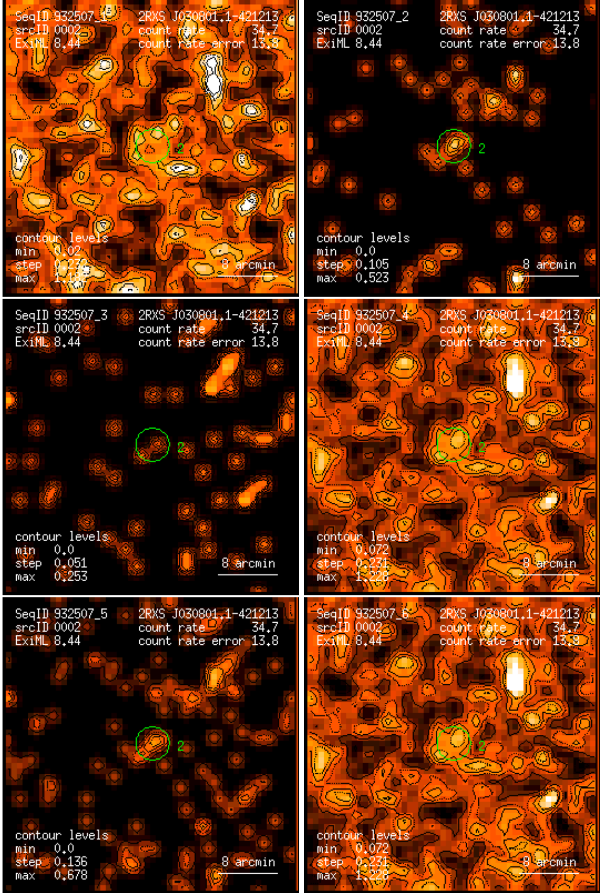
Figure 2: RASS 932507: detection 0002: band rate images, Gaussian filter: (1) PSPC channels 11 – 41, (2) 52 – 90, (3) 91 – 201, (4) 11 – 235, (5) 52 – 201, (6) 11 – 201. Broad band rates in counts/ks. Band rate contour levels in counts/ks/arcmin 2 .
