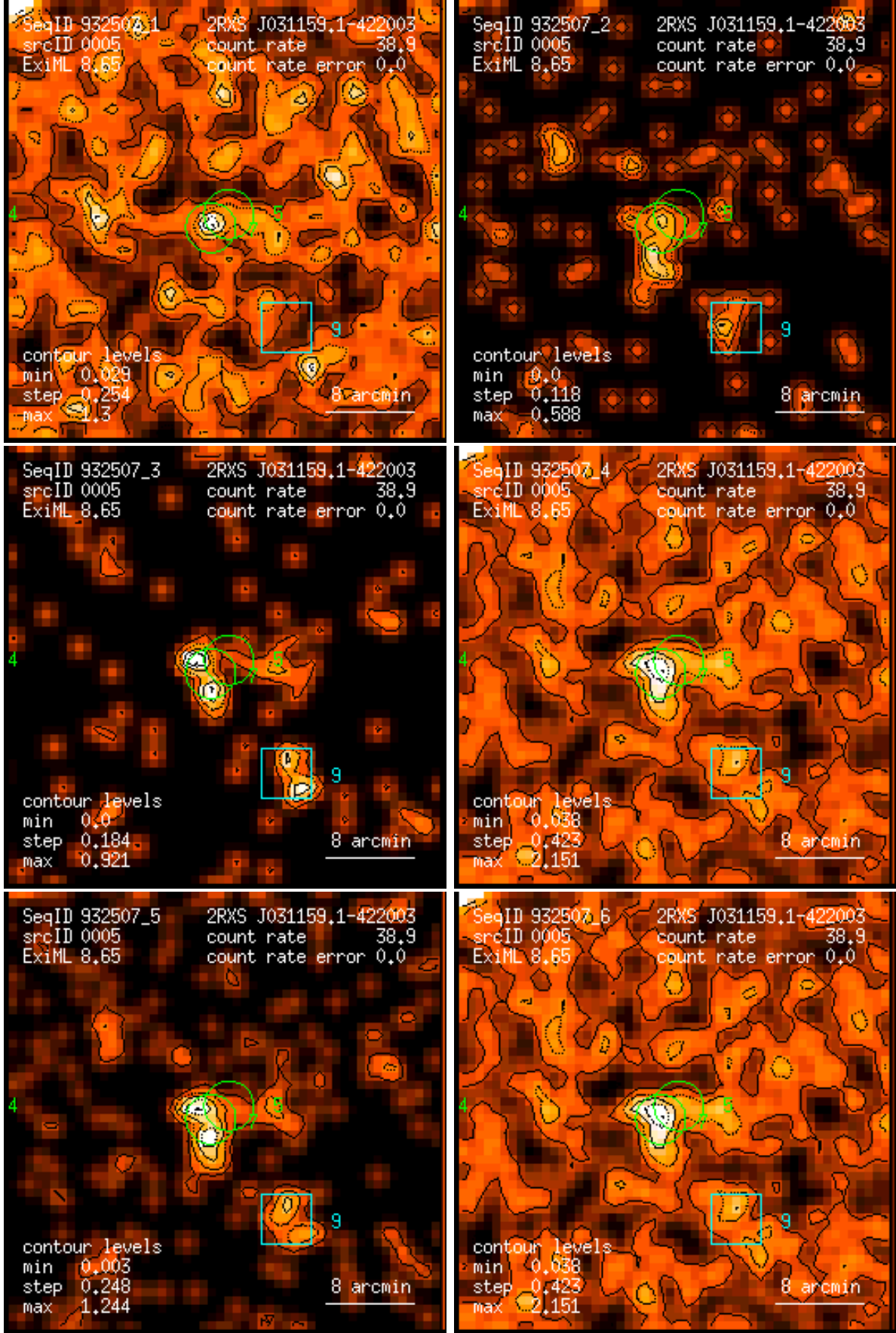
Figure 5: RASS 932507: detection 0005: band rate images, Gaussian filter: (1) PSPC channels 11 – 41, (2) 52 – 90, (3) 91 – 201, (4) 11 – 235, (5) 52 – 201, (6) 11 – 201. Broad band rates in counts/ks. Band rate contour levels in counts/ks/arcmin 2 .
