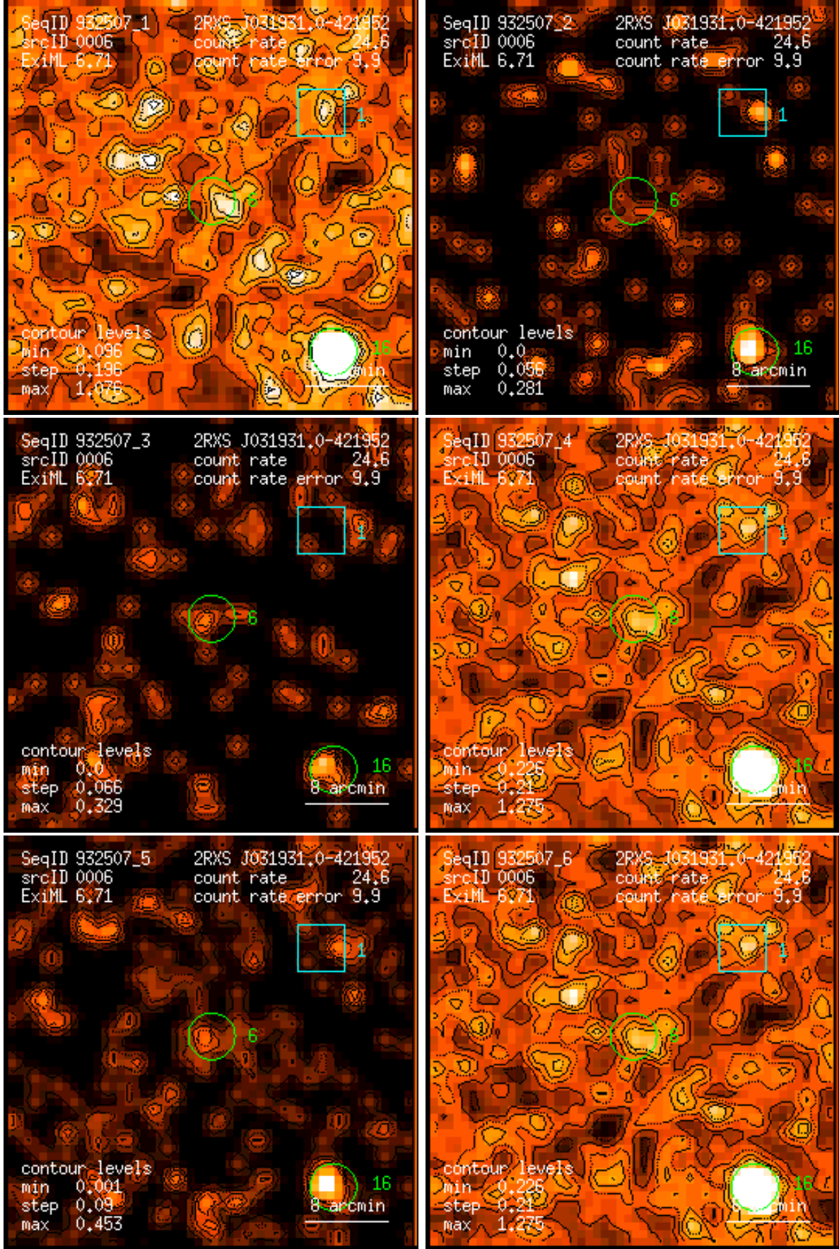
Figure 6: RASS 932507: detection 0006: band rate images, Gaussian filter: (1) PSPC channels 11 – 41, (2) 52 – 90, (3) 91 – 201, (4) 11 – 235, (5) 52 – 201, (6) 11 – 201. Broad band rates in counts/ks. Band rate contour levels in counts/ks/arcmin 2 .
