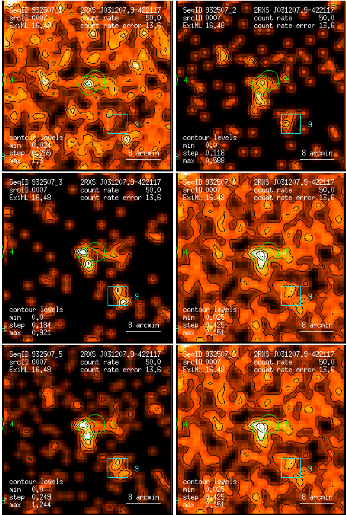
Figure 7: RASS 932507: detection 0007: band rate images, Gaussian filter: (1) PSPC channels 11 – 41, (2) 52 – 90, (3) 91 – 201, (4) 11 – 235, (5) 52 – 201, (6) 11 – 201. Broad band rates in counts/ks. Band rate contour levels in counts/ks/arcmin 2 .
