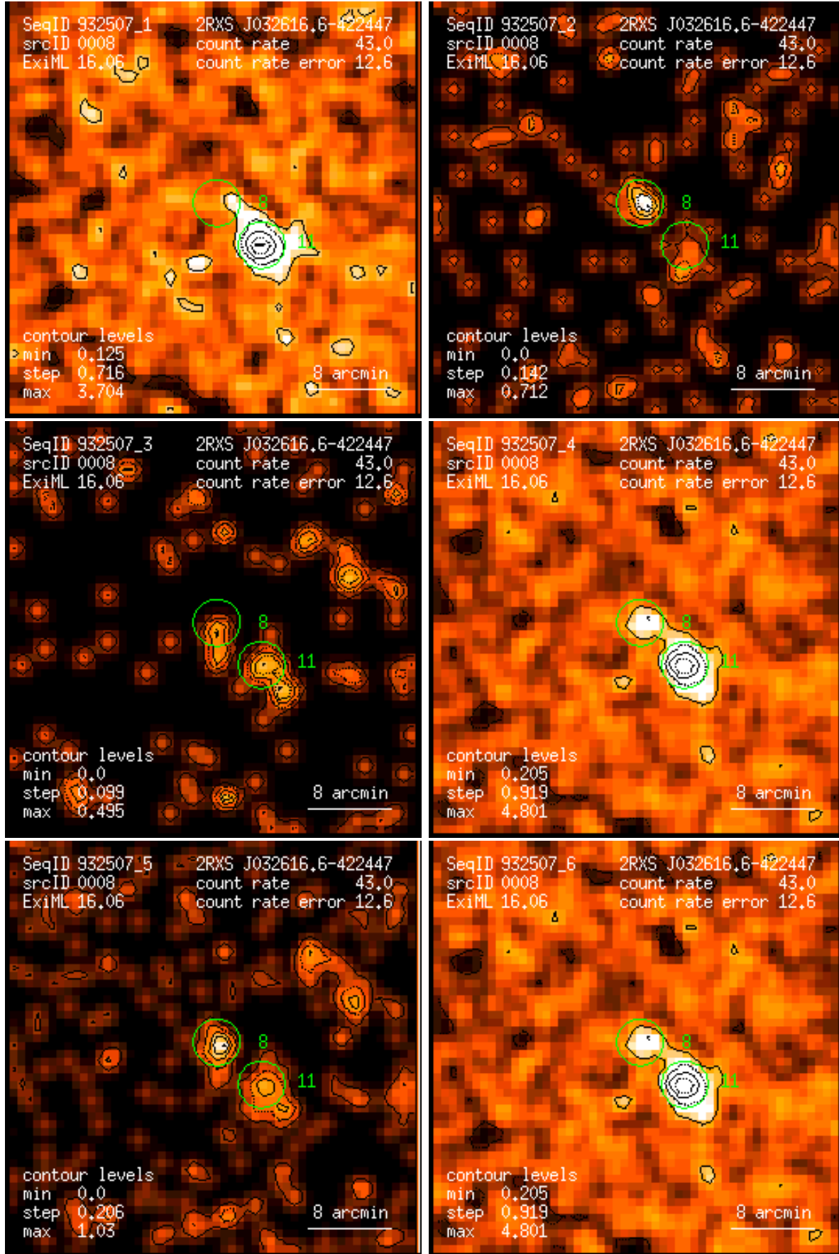
Figure 8: RASS 932507: detection 0008: band rate images, Gaussian filter: (1) PSPC channels 11 – 41, (2) 52 – 90, (3) 91 – 201, (4) 11 – 235, (5) 52 – 201, (6) 11 – 201. Broad band rates in counts/ks. Band rate contour levels in counts/ks/arcmin 2 .
