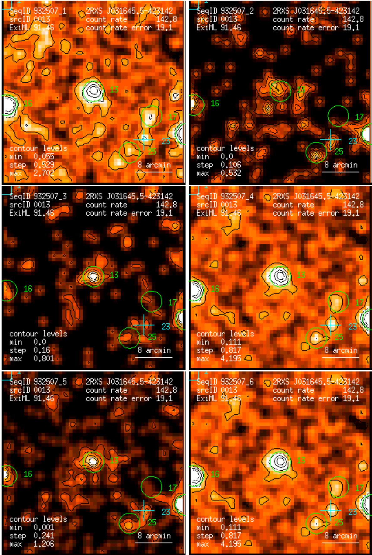
Figure 13: RASS 932507: detection 0013: band rate images, Gaussian filter: (1) PSPC channels 11 – 41, (2) 52 – 90, (3) 91 – 201, (4) 11 – 235, (5) 52 – 201, (6) 11 – 201. Broad band rates in counts/ks. Band rate contour levels in counts/ks/arcmin 2 .
