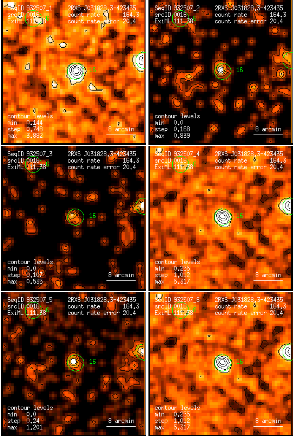
Figure 16: RASS 932507: detection 0016: band rate images, Gaussian filter: (1) PSPC channels 11 – 41, (2) 52 – 90, (3) 91 – 201, (4) 11 – 235, (5) 52 – 201, (6) 11 – 201. Broad band rates in counts/ks. Band rate contour levels in counts/ks/arcmin 2 .
