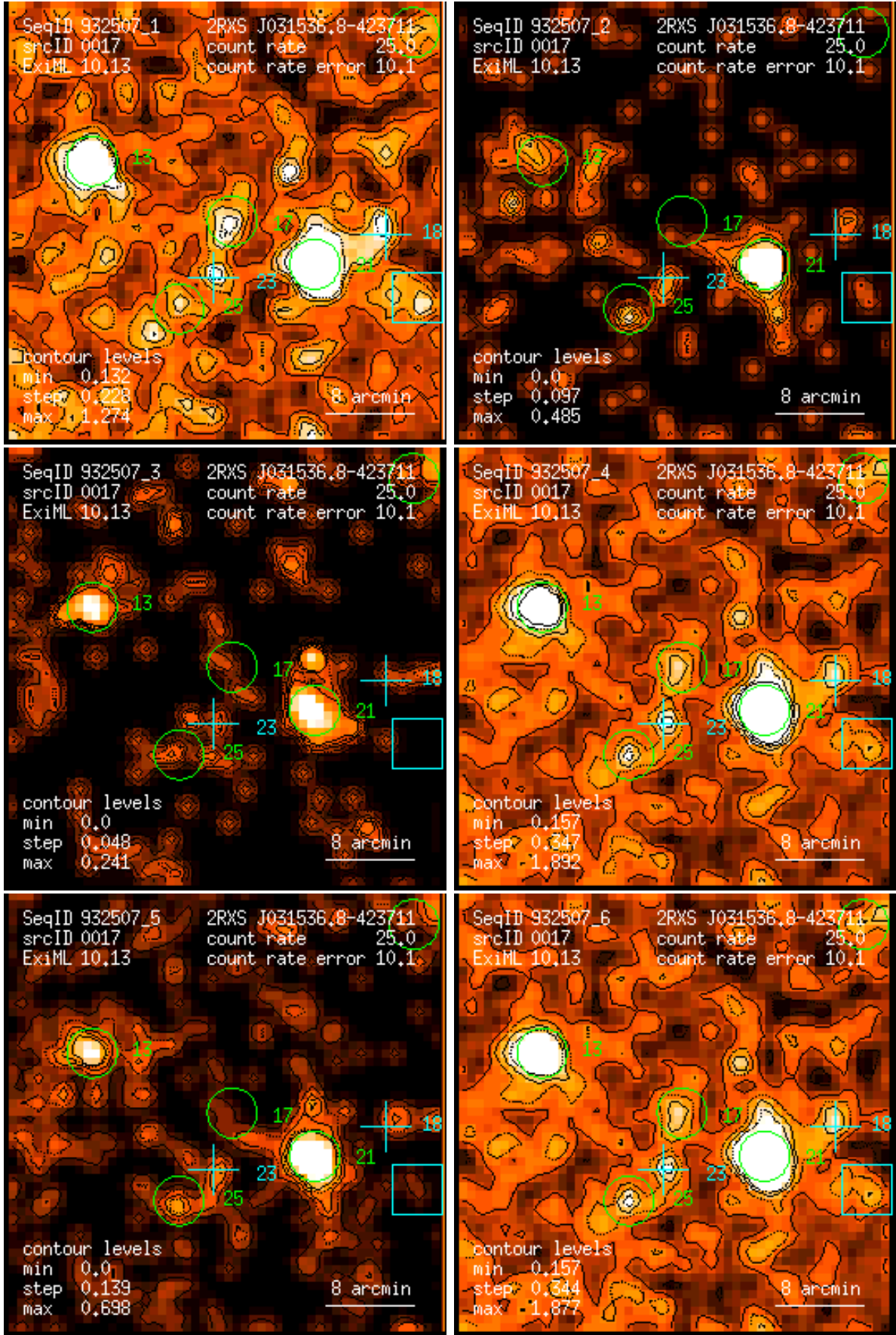
Figure 17: RASS 932507: detection 0017: band rate images, Gaussian filter: (1) PSPC channels 11 – 41, (2) 52 – 90, (3) 91 – 201, (4) 11 – 235, (5) 52 – 201, (6) 11 – 201. Broad band rates in counts/ks. Band rate contour levels in counts/ks/arcmin 2 .
