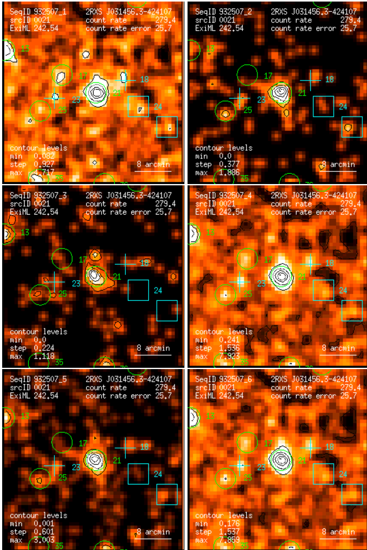
Figure 21: RASS 932507: detection 0021: band rate images, Gaussian filter: (1) PSPC channels 11 – 41, (2) 52 – 90, (3) 91 – 201, (4) 11 – 235, (5) 52 – 201, (6) 11 – 201. Broad band rates in counts/ks. Band rate contour levels in counts/ks/arcmin 2 .
